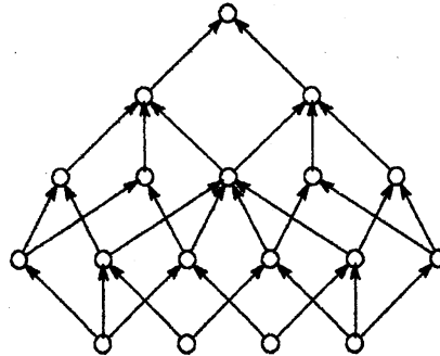
Figure 8: semilattice 12564
