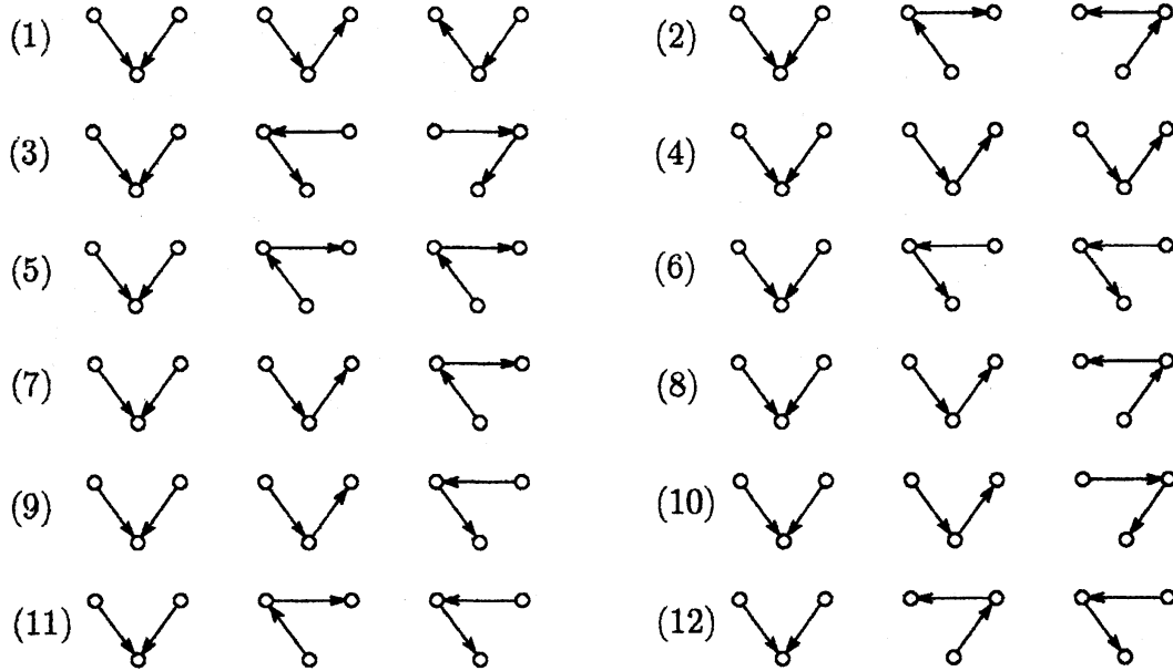
Figure 4: VII type
