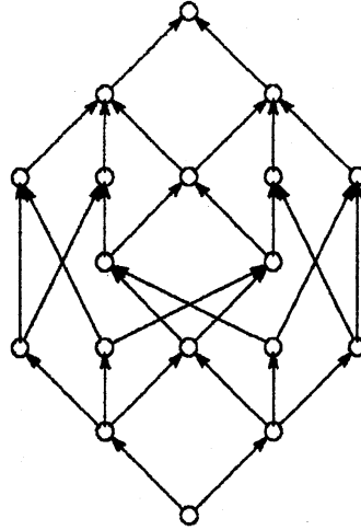
Figure 9: semilattce 1252521
