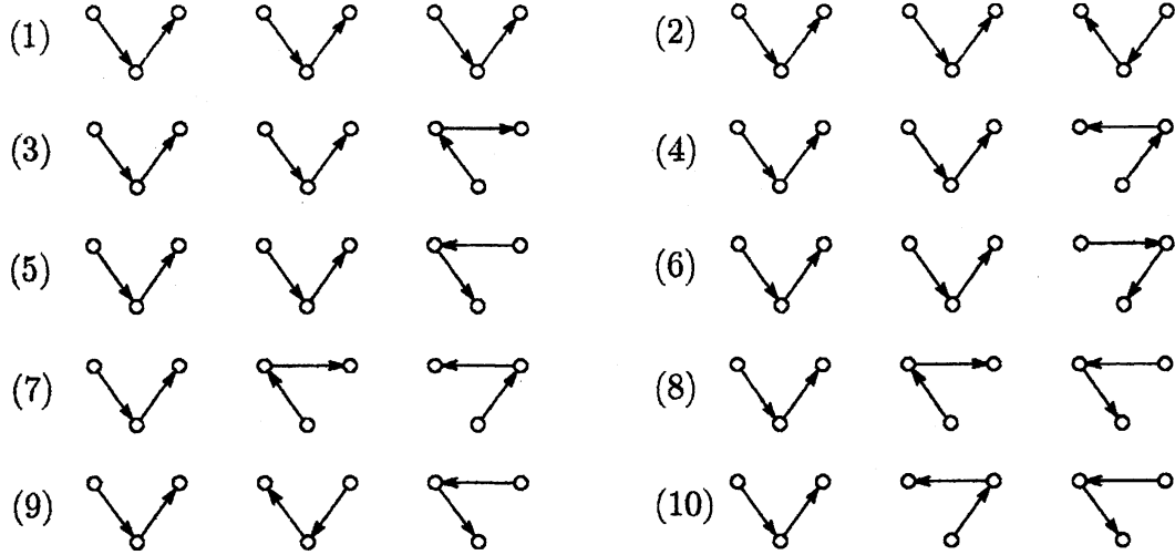
Figure 3: III type
