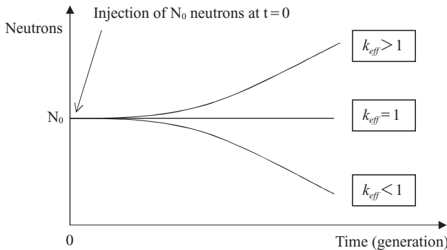
Fig. 1-2 Time evolution of neutrons
