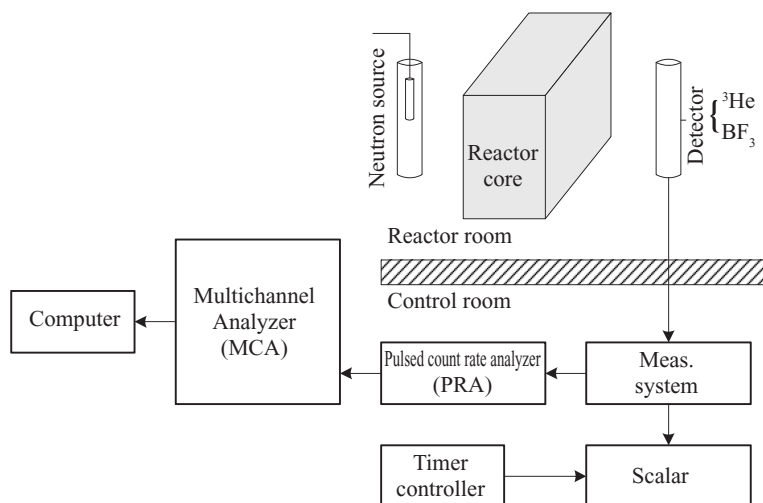
Fig. 4-4 Measurement system
