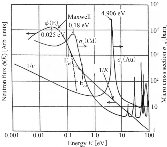
Fig. 3-4 Neutron spectrum in the thermal reactor and energy dependence of all the cross sections of Cd and Au
