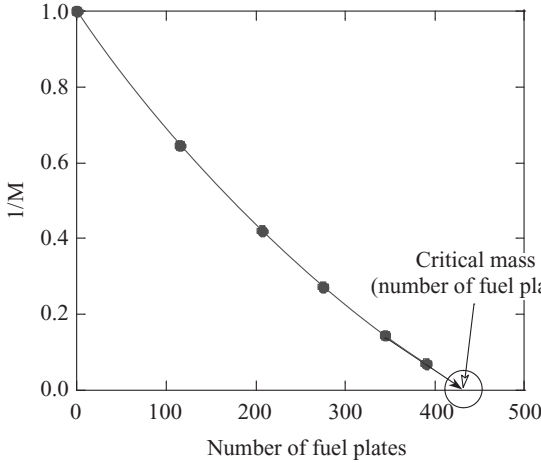
Fig. 1-3 Plot of 1/M versus fuel mass (number of fuel plates)
