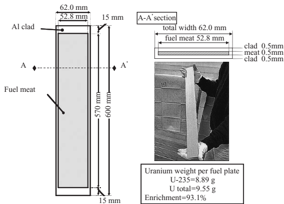
Fig. 8 Fuel plate
