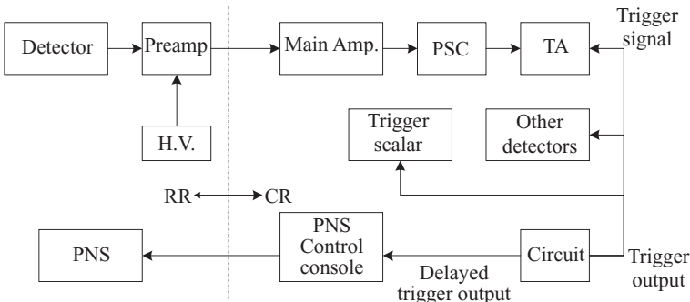
Fig. 5-4 Measurement system
