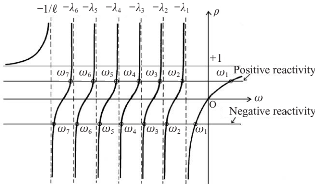
Fig. 2-1 Relation between reactivity \rho and \omega
