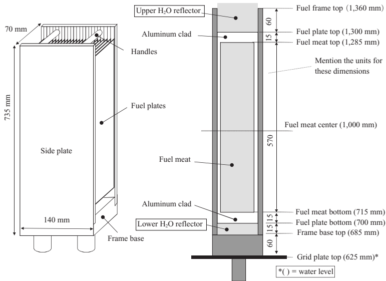
Fig. 9 Fuel frame
