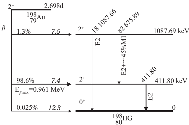
Fig. 3-1 Disintegration of ^{198}\text{Au}
