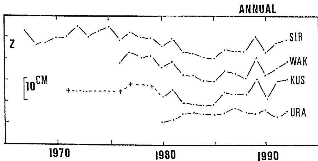
Fig. 4 Interannual variations of the annual means of the tide levels at the tide stations; Shirahama (SIR), Wakayama (WAK), Kushimoto (KUS) and Urugami (URA).
