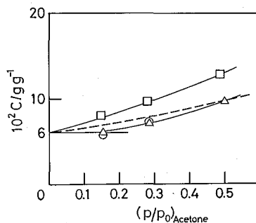
Fig. 5. Sorption isotherms of the system of acetone/normal-hexane mixtures and the slightly cross-linked PB at 25°C and at p=4.85 cmHg of n -hexane. Absorption runs were made in three ways: acetone first (○), n -hexane first (□), and simultaneously (△). A dashed line was calculated by assuming simple additivity in equilibrium concentration of the penetrant.
