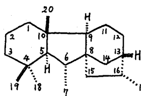
Gibberellane
