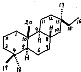
Pimarane
