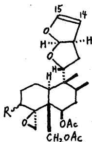
(147a) R = \beta-OAc
