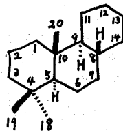
Podocarpane
