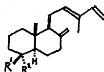
(43) R^1 = \text{COOH} , R^2 = \text{Me}
