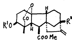
(388) R 1 = Ac, R 2 = OH
