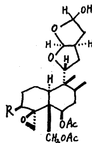
(147c) R = OAc
