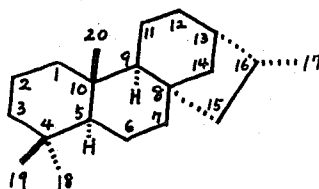
Kaurane
