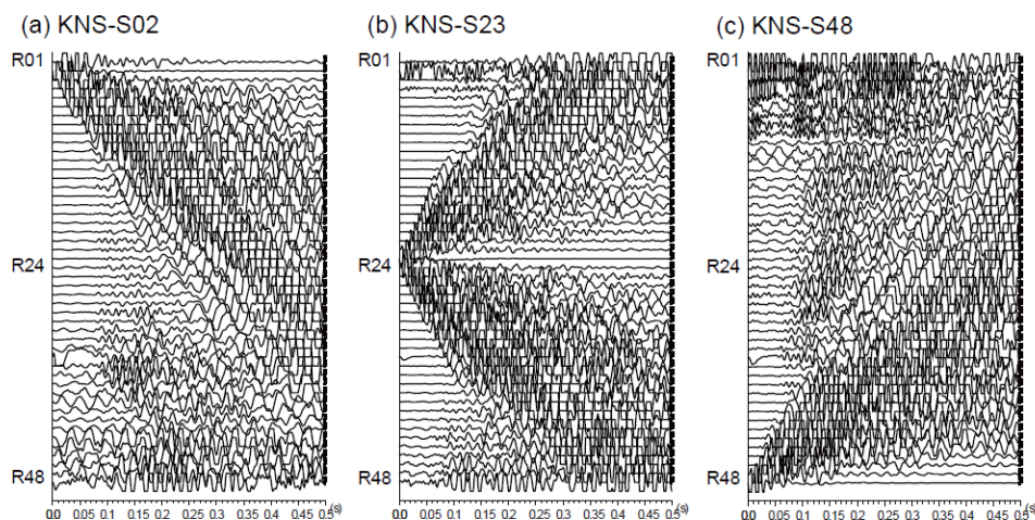
Fig. 9 Filtered shot records along the line KNS with BPF 10 – 100 Hz.
