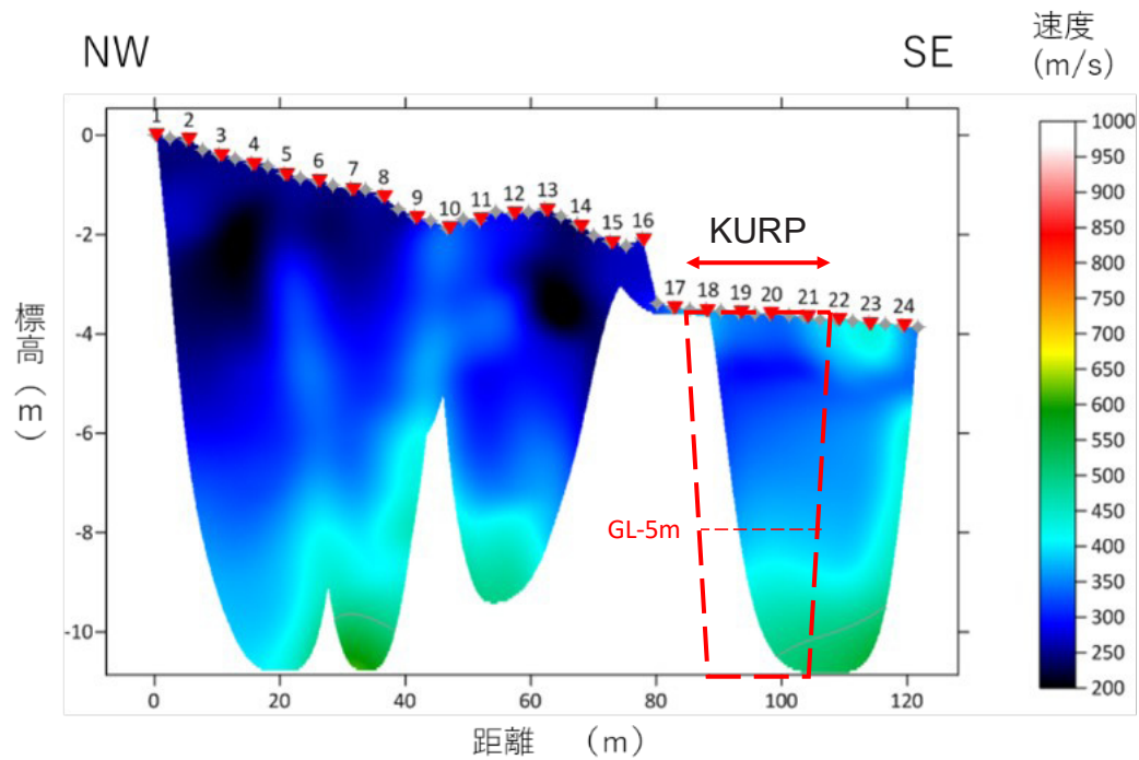
Fig. 16 Velocity structure beneath the line KUR as a result of the smooth inversion in RAYFRACT. The excavation for KURP is indicated a broken red trapezoid. The shot points are red triangles. Gray diamonds are the receivers
