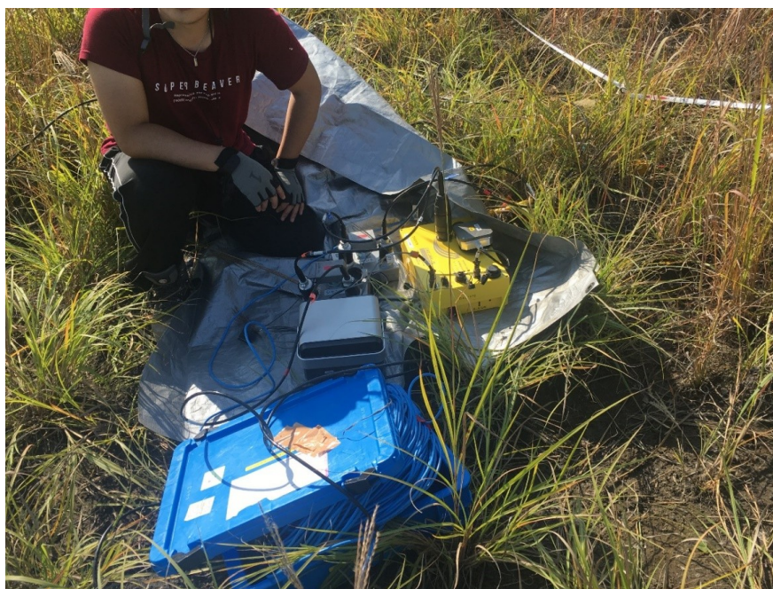
Fig. 8 Seismic data acquisition system DAQ Link 3 in operation.
