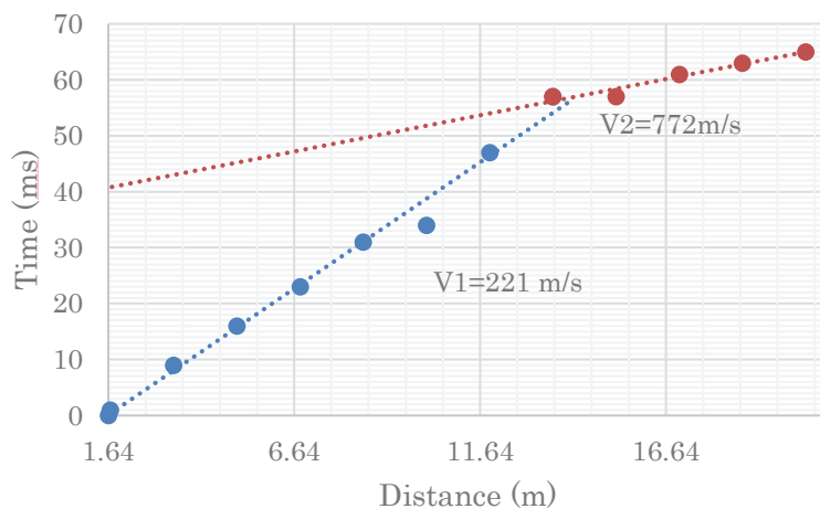
Fig. 12 Travel time curve from the shot at 1.7 m.
