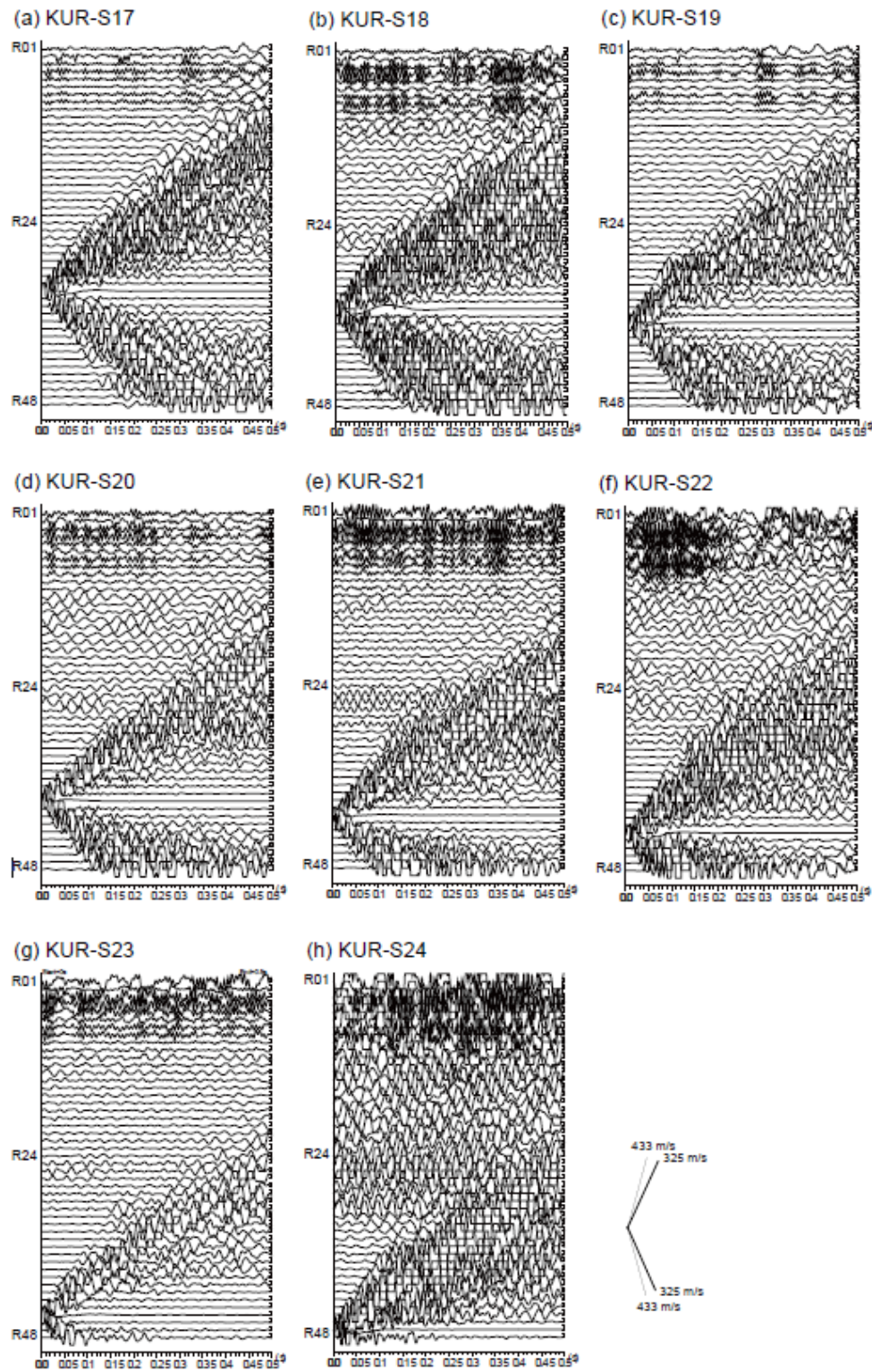
Fig. 10 Filtered shot records across the excavation area KURP along the line KUR with 10-100 Hz BPF.
