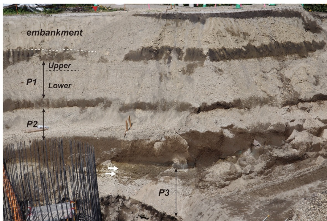
Fig. 3 The cross section of the excavation on north side.
