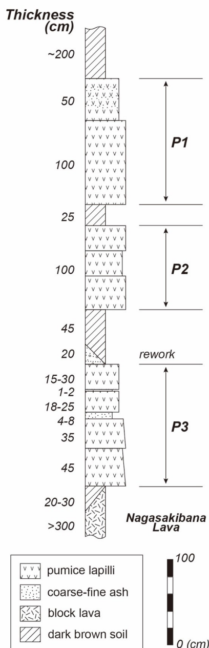
Fig. 4 Schematic stratigraphic column at the excavation KURP.
