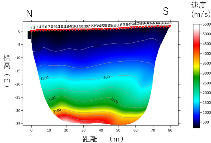
Fig. 15 Velocity structure in the line KNS as a result of smooth inversion in RAYFRACT. The shot points are red triangles. Gray diamonds are the receivers.
