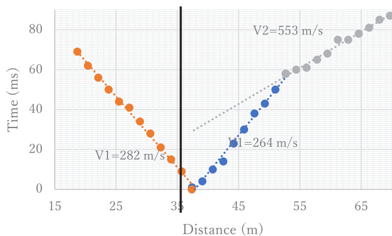
Fig. 13 Travel time curve from the shot at 37 m.
