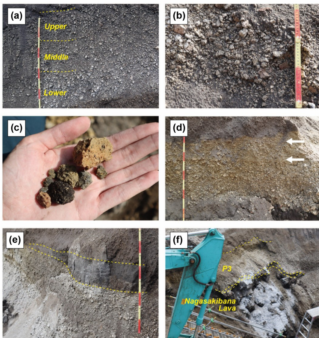
Fig. 5 (a) A close-up view of P2. (b) Abundant reddish pumices in the base of P2. (c) A variety of pumices in P3. (d) A close-up view of P3. White arrows show ash layers. (e) Coarse sand layer overlying P3. (f) 769's lava (Nagasaki-bana lava) covered by P3. Thickness of P3 is about one meter.
