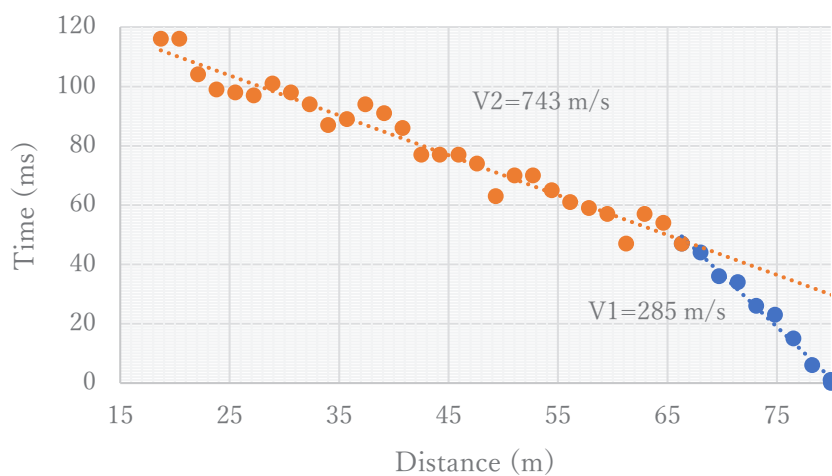
Fig. 14 Travel time curve from the shot at 79 m.
