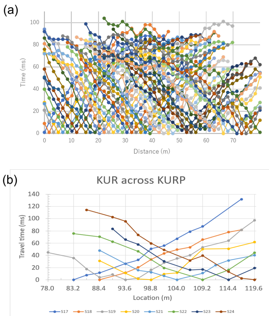
Fig. 11 Travel time curves. a) Line KNS. b) Line KUR in the excavation zone. Good quality picks were plotted.
