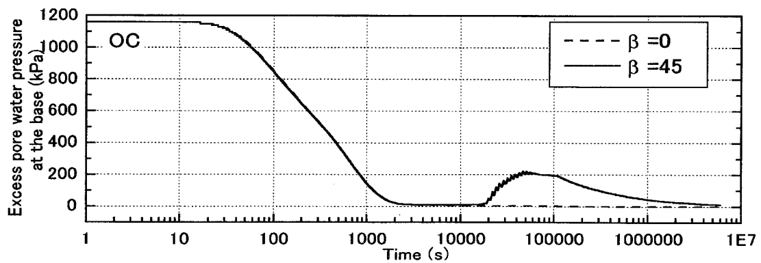
Figure 4.22: Generated pore water pressure for OC clay
