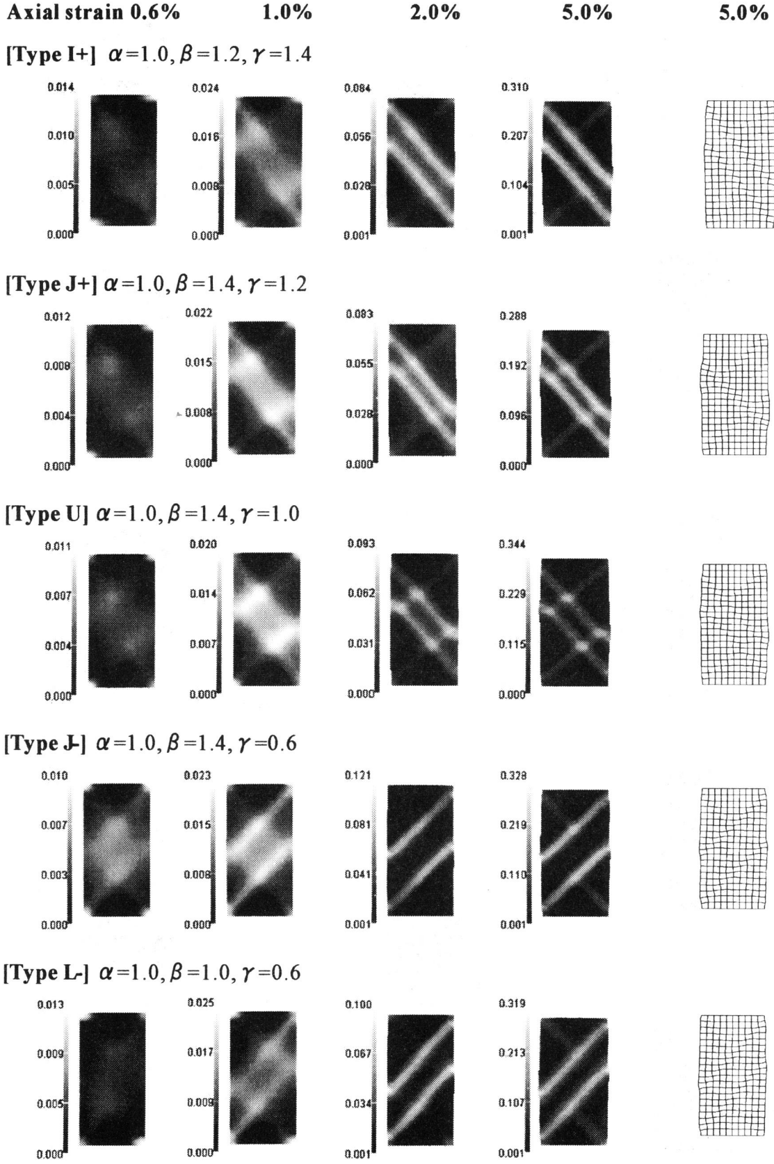
Figure 6.7: (a) Distribution of viscoplastic deviatoric strain and deformed meshes (\theta = 30^\circ)
