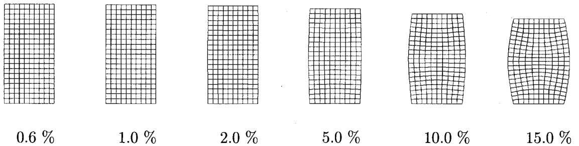
Figure 3.73: Deformed meshes for OC clay ( \beta=0 , Drained))
