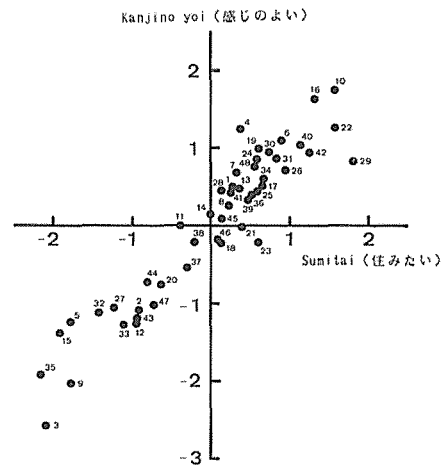
Fig. 11 Relation between "Sumitai" or "want to live" and "Kanjino yoi" or "agreeable". 「住みたい」と「感じのよい」の関係
