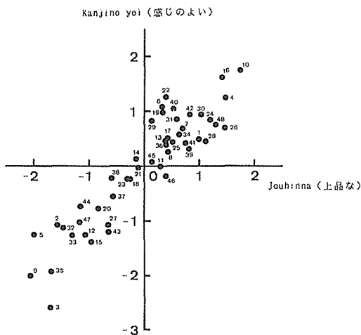
Fig. 10 Relation between "Jouhinna" or "elegant" and "Kanjino yoi" or "agreeable". 「上品な」と「感じのよい」の関係
