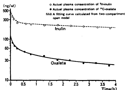
Fig. 3. Semilogarithmic plots of actual plasma concentrations of oxalate and inulin against time and the fitting curves obtained on the basis of two-compartment open model in nephrectomized rat.
