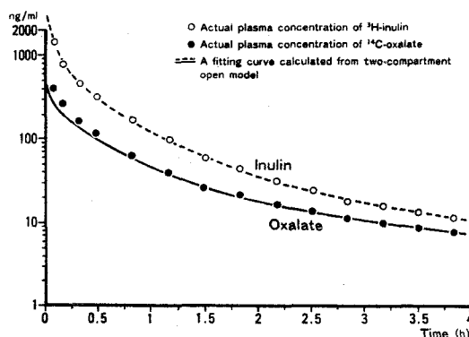
Fig. 2. Semilogarithmic plots of actual plasma concentrations of oxalate and inulin against time and the fitting curves obtained on the basis of two-compartment open model in normal rat.
