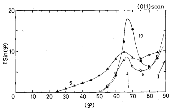
Fig. 7. \sin \phi I(\phi) vs. \phi for (011). See the legend for Fig. 4 for triangles, circles and arrows.
