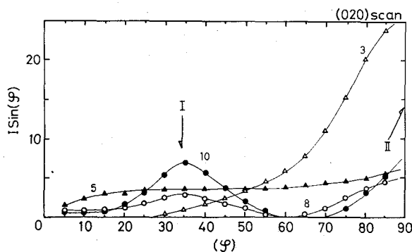
Fig. 6. \sin \phi I(\phi) vs. \phi for (020). See the legend for Fig. 4 for triangles, circles and arrows.
