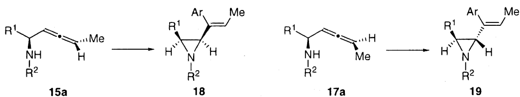
Scheme 4. Reaction conditions: cat. \text{Pd}(\text{PPh}_3)_4 , Ar-I, \text{K}_2\text{CO}_3 , dioxane, reflux.
