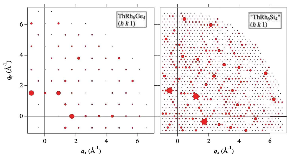
Fig. 1. X-ray diffraction data for ThRh_6Ge_4 and “ ThRh_6Si_4 ”.
