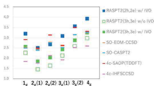
Fig. 1. Vertical excitation energies of \text{UO}_2^{2+} molecule
