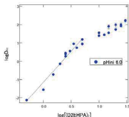
Fig. 1. Dependence of \log D_{\text{Ac}} vs. \log[(\text{D2EHPA})_2]
