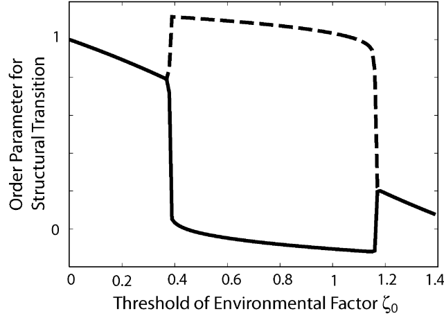
Figure 7. Bifurcation diagram of the system with equations (2.4) - (2.7) with a change in the threshold of environmental factor \zeta_0 . The vertical axis shows the maximum and minimum amplitudes of the oscillation generated by this system. For stable oscillation in this system, there is a proper region of the threshold for the environmental factor \zeta_0 .
