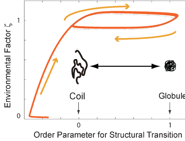
Figure 6. Dynamics in phase space ( \eta - \zeta plane) of the result shown in Fig. 5. The limit-cycle orbit is shown, with flow drawn with arrows.
