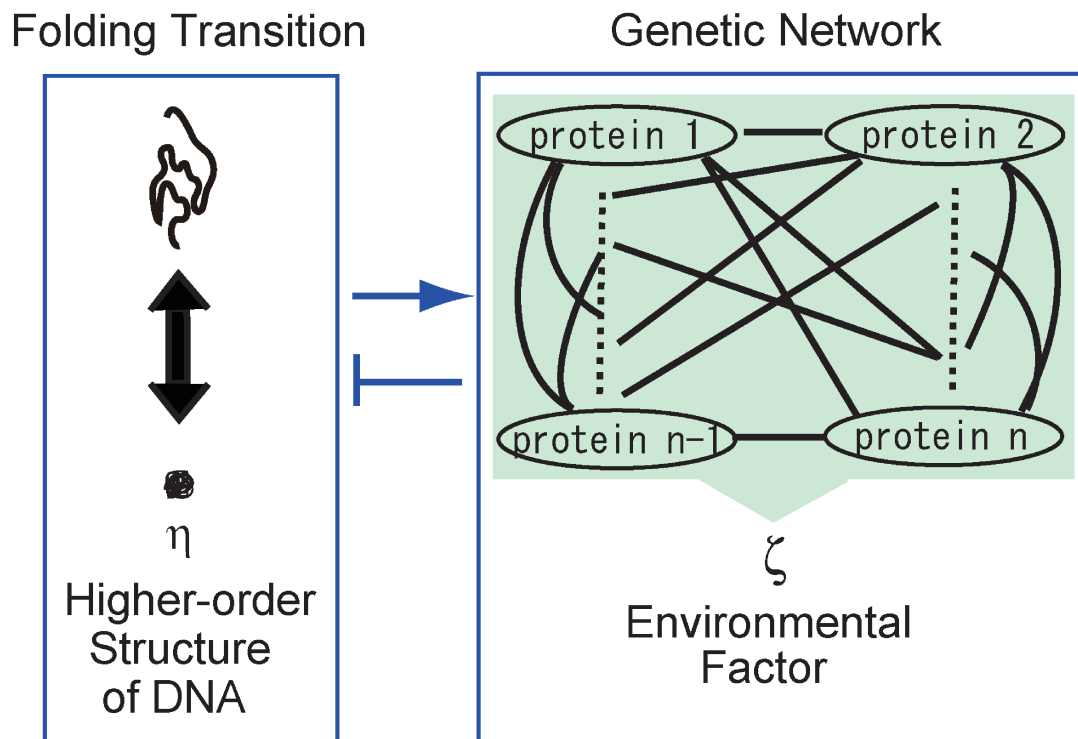
Figure 4. Interaction between DNA conformation and an environmental factor. When a DNA molecule is in the coiled state, its transcriptional activity is “on” and proteins transcribed from mRNA suppress the transcriptional activity of DNA by changing the free-energy profile of DNA; the DNA molecule is folded through the environmental factor ( \zeta ). The transcriptional activity of DNA then turns off and neither mRNA nor proteins are produced, until the DNA molecule becomes unfolded again. This is the mechanism of self-regulation which includes the folding transition of DNA.
