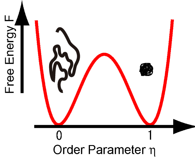
Figure 3. Free-energy profile of a DNA molecule with a size of over several tens of kbp. A simple bimodal profile is adopted to describe the intrinsic nature of the discrete structural transition in a giant DNA molecule. The order parameter \eta corresponds to the segment density of DNA: \eta = 0 and \eta = 1 indicate the coiled and compact states, respectively.
