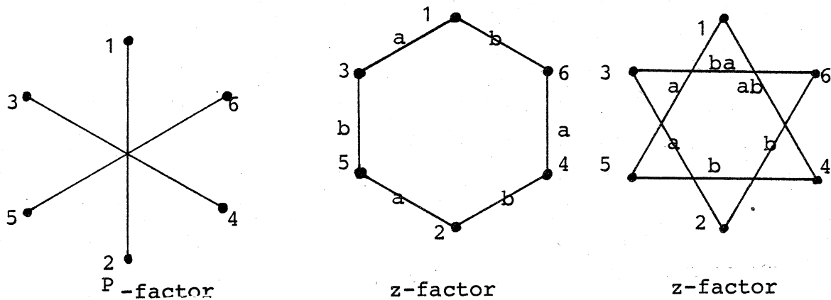
Fig. 3. Examples of factorization.
