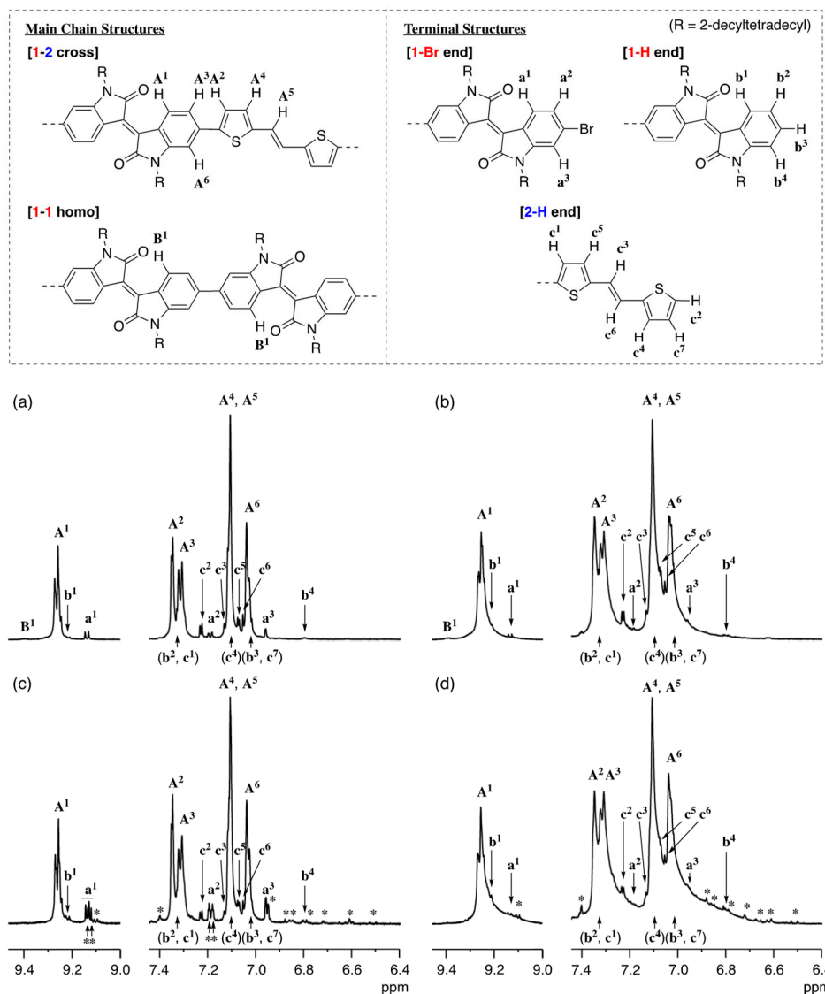
Figure 1. 1 H-NMR spectra of poly(1-alt-2) prepared via DArP ( M_n = 15,700 (a) and M_n = 22,700 (b)) and Migita–Kosugi–Stille cross-coupling polymerization ( M_n = 17,700 (c) and M_n = 24,400 (d)) in C 2 D 2 Cl 4 at 130 °C (600 MHz). *: unidentified signals.
