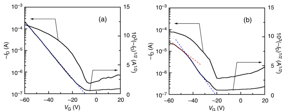
Figure 3. Charge transfer characteristics of the OFETs using poly(1- alt -2) of entries 1 (a) and 5 (b) in Table 3 ( V_D = -60 V).
