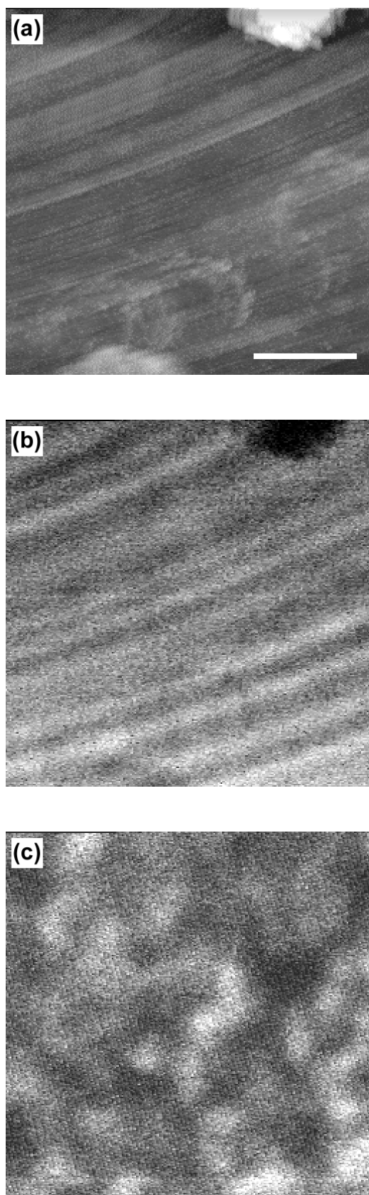
Figure 5.2. Topographic (a), transmission (b), and fluorescence SNOM images (c) for the side-chain labeled PMMA network with a crosslink density of 0.1 %. All the images were obtained for the same area. The wavelength of the light source was 442 nm. The scale bars indicate 1 \mu\text{m} .
