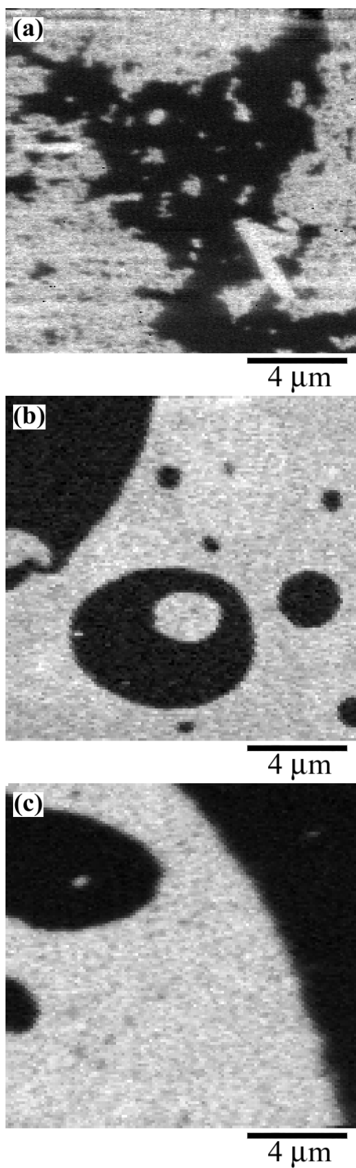
Figure 4.5. Perylene fluorescence SNOM images for the PODMA-Pe / PiBMA-Py monolayers with different annealing times; (a) 0, (b) 5, and (c) 60 min. The excitation wavelength was 442 nm and the fluorescence from perylene was collected through a filter, SC-46 (Fuji).
