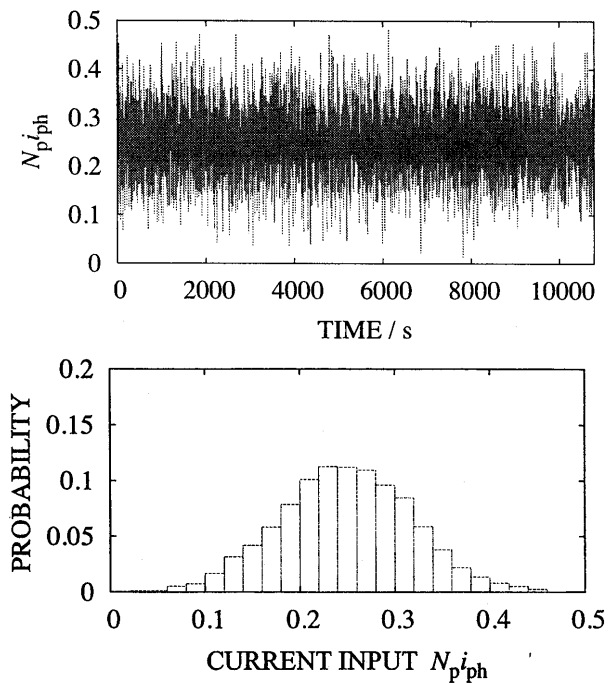
Fig. 8 One example of time series and probability density of uncertain input from the photoelectric current of the PV array. The time series is generated as a Gaussian distribution.
