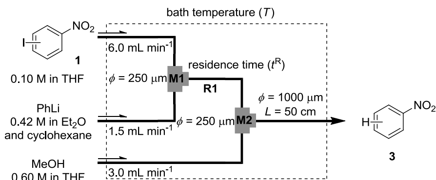
Figure 1. A microreactor system for the I-Li exchange reaction of iodonitrobenzenes 1 followed by reaction with MeOH.
