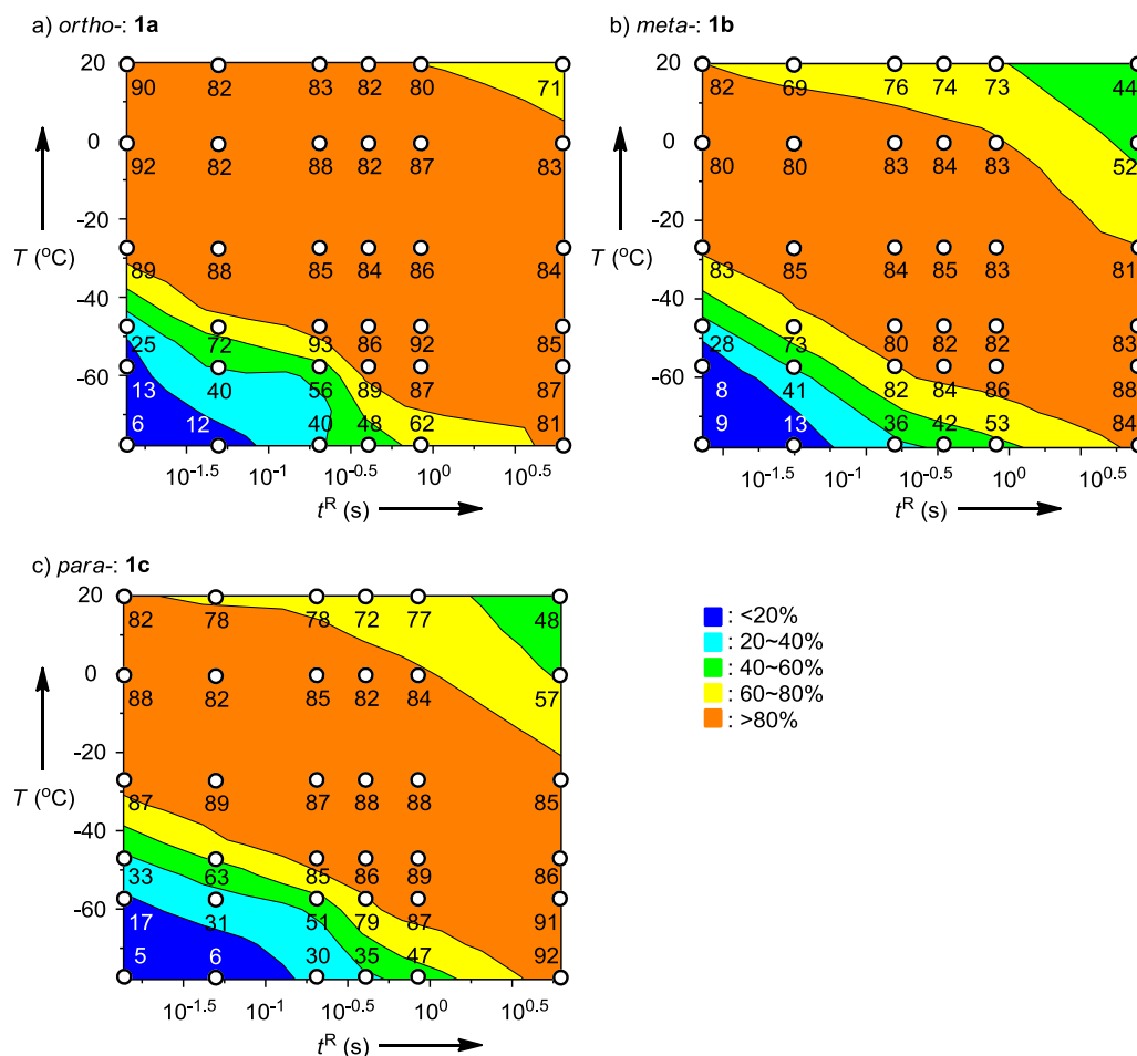
Figure 2. Effect of the temperature and the residence time on the yield of 3 in the Br-Li exchange reaction of a) o -bromobenzonitrile ( 1a ), b) m -bromobenzonitrile ( 1b ), c) p -bromobenzonitrile ( 1c ) in flow microreactor systems.
