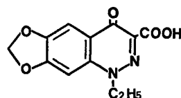
Fig. 1. Chemical structure of cinoxacin
