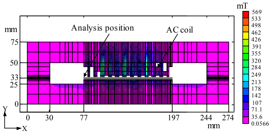
Fig. 3.2 The distribution of magnetic flux density with AC current at 6 A_{peak} in the iron core. The analysis position is also shown as a line.
