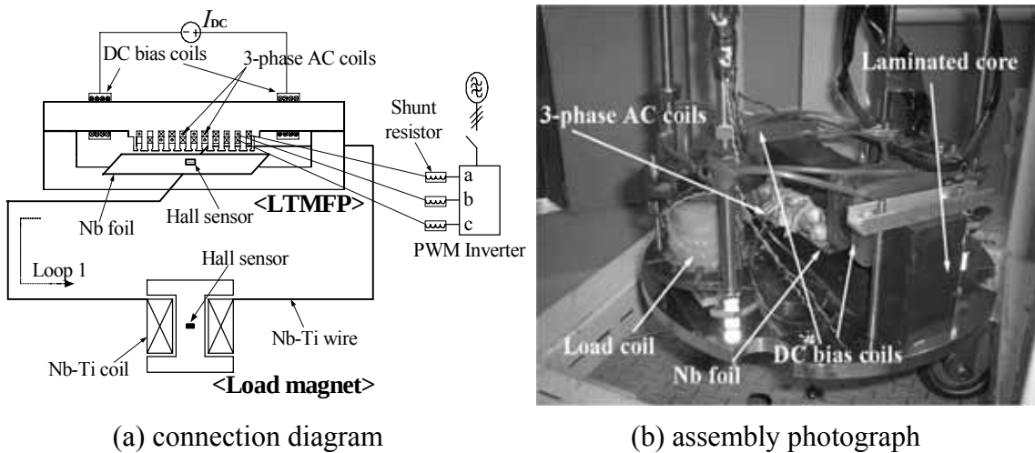
Fig. 5.3 Current pumping system with small-scale load magnet (1.3 mH).
