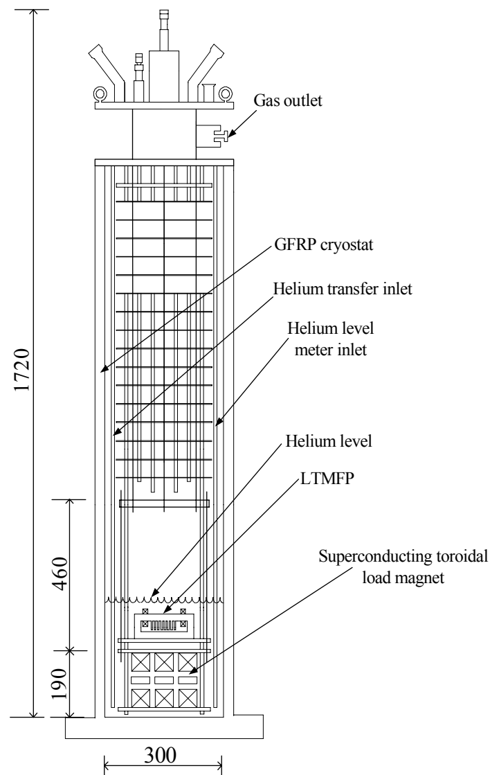
Fig. 5.2 Inner structure of the GFRP cryostat.
