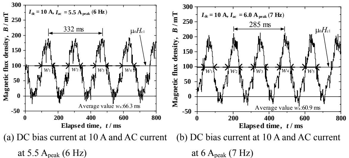
Fig. 5.5 Temporal variation of the magnetic flux density at the central part in the air gap. The measured temperature is 4.2 K.
