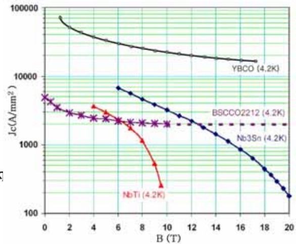
(b) critical current density J_c versus magnetic flux density B
