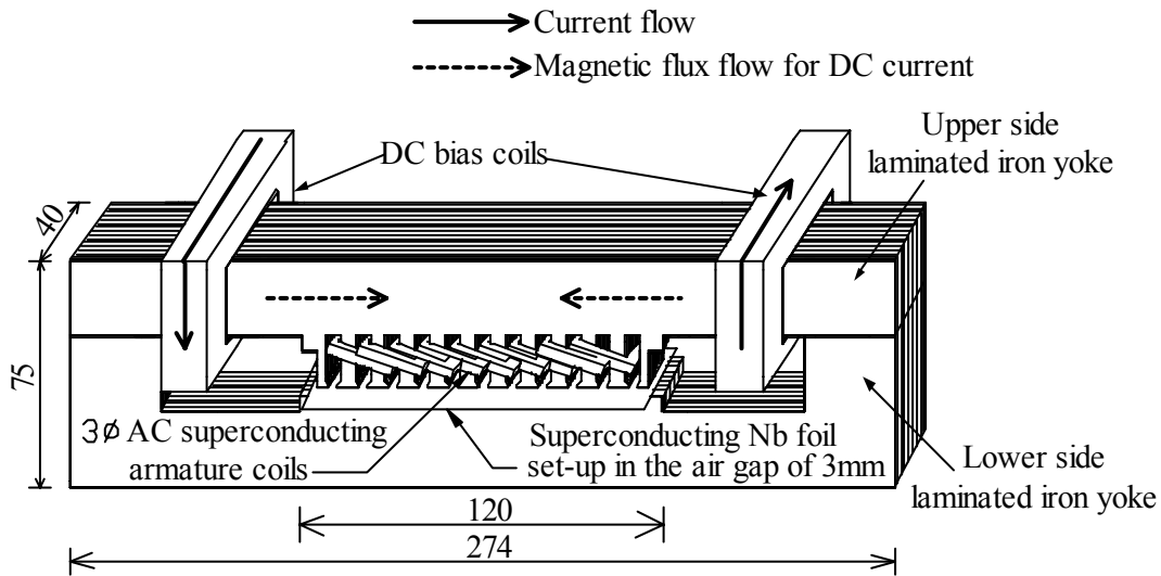
Fig. 4.2 Schematic diagram of the LTMFP (unit: mm).
