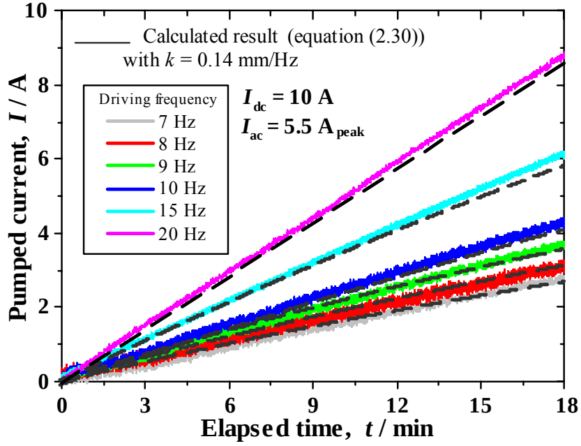
Fig. 5.11 Measured and calculated results of the pumped current with DC bias current at 10 A and AC current at 5.5 A peak . The measured temperature is 4.2 K.
