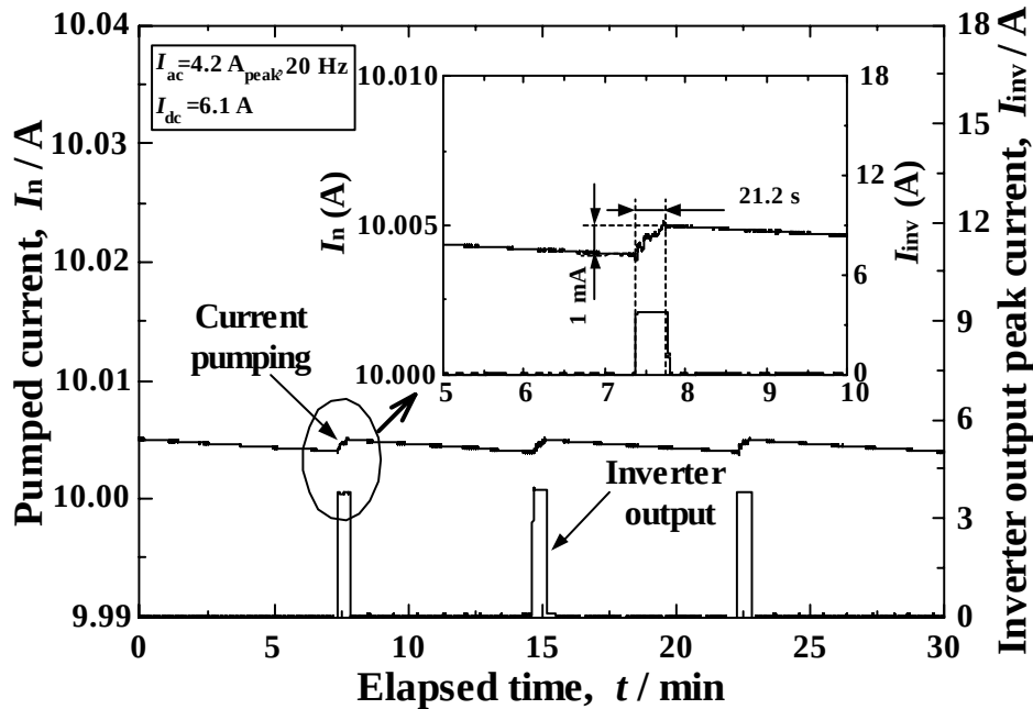
Fig. 6.12 Current Compensation of superconducting toroidal magnet by means of LTMFP with the condition of DC bias current at 6.1 A and AC current at 4.2 A peak (20 Hz).
