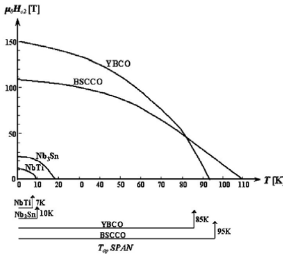
(a) typical upper critical magnetic field \mu_0 H_{c2} versus temperature T plots
