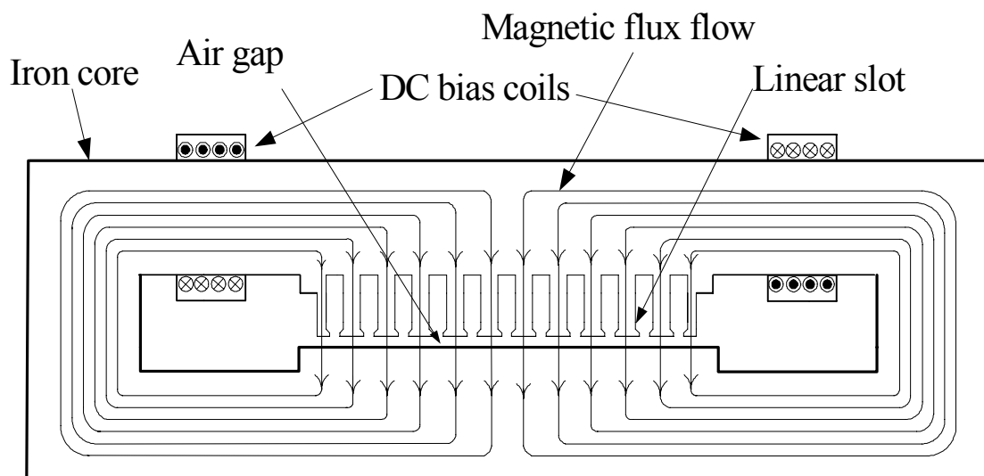
Fig. 4.6 Schematic diagram of the magnetic flux flow by DC bias currents.
