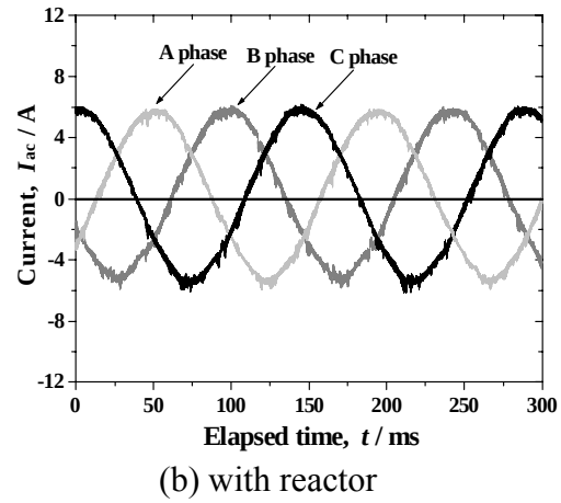
Fig. 5.9 Current waveforms of the 3-phase inverter at 6 A peak (7 Hz) at room temperature.
