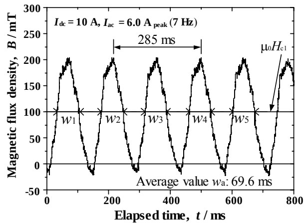
Fig. 5.10 Temporal variations of the magnetic flux density at the central part in the air gap with 3-phase reactor. The driving frequency is 7 Hz and the measured temperature is 4.2 K.
