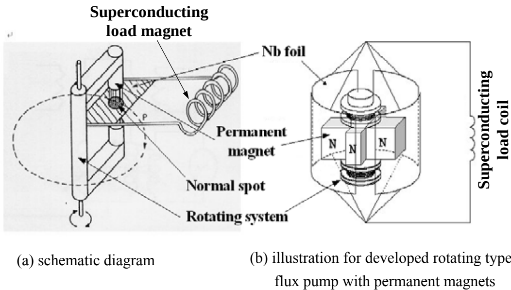
Fig. 2.1 Principle of rotating-type superconducting flux pump [65].
