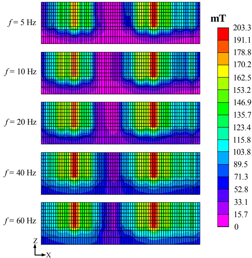
Fig. 3.9 Contour plots of the magnetic flux density in the Nb foil for different driving frequencies with the DC bias current at 10 A and the AC current at 6 A peak . The upper surface is the symmetrical plane of the upper part. The electrical angle of the A-phase is 120°.
