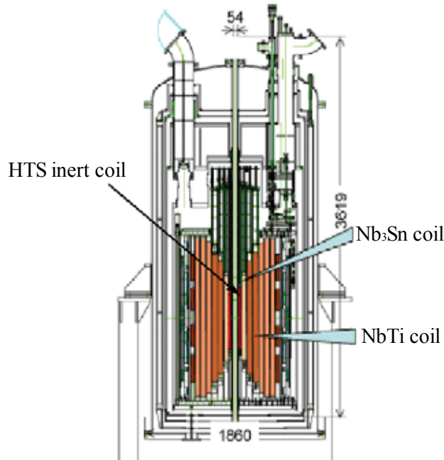
Fig. 1.7 Schematic sectional view of NMR spectrometer magnets [30].
