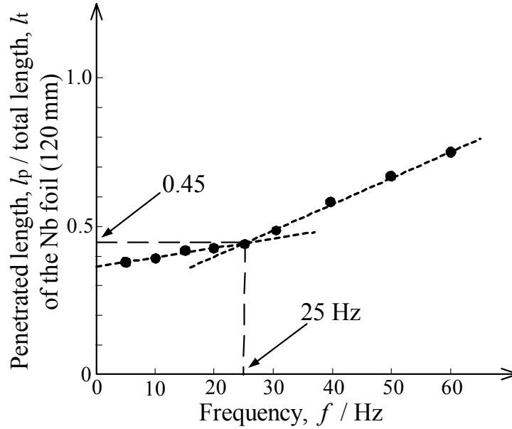
Fig. 3.11 Calculated results of the invaded magnetic flux normalized by the total length of the Nb foil (120 mm). The criterion for the definition of the invaded area is 100 mT ( \mu_0 H_{c1} ).
