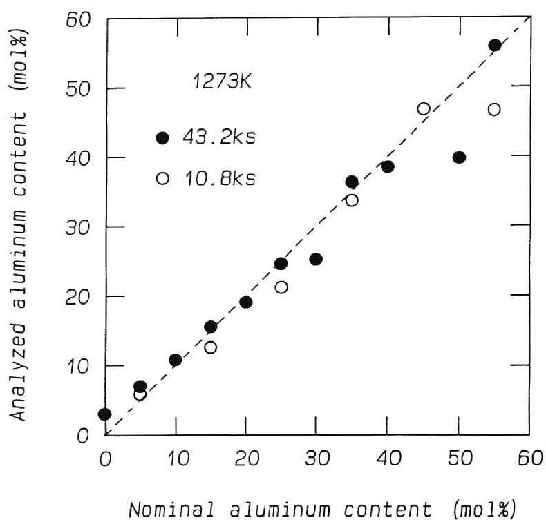
Figure 3.7: Analyzed aluminum concentration against the nominal aluminum compositions in the starting oxide mixture. The nominal compositions are shown as the ratio of \text{Al}/(\text{Al}+\text{Ti}) . The open and closed circles show the analyzed values of the specimens reduced at 1273K for 10.8 ks and 43.2 ks.
