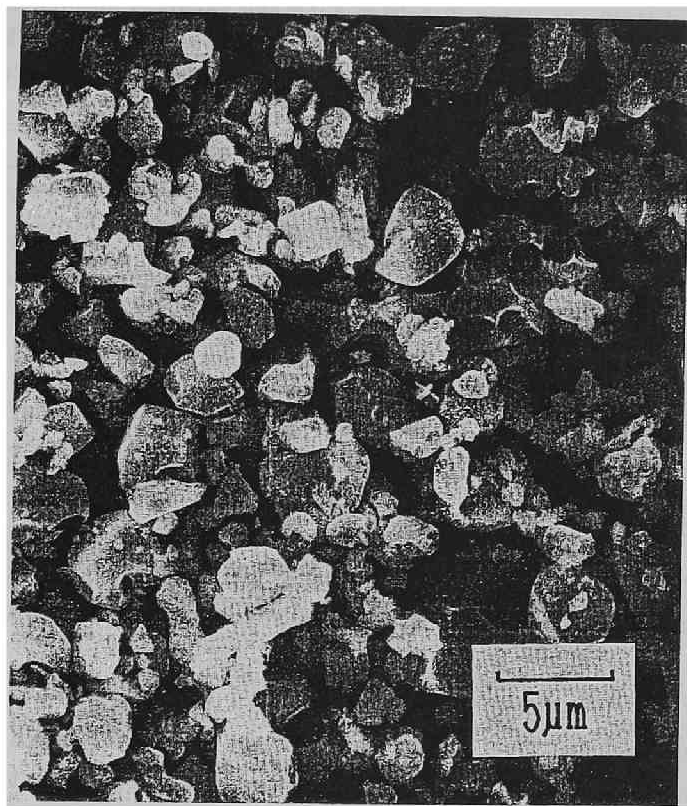
Figure 4.3: Scanning electron micrograph of \text{TiAl}_3 powders reduced by \text{CaH}_2 for 10.8 ks at 1273K. The molar ratio of Al:Ti in the starting oxide mixture was 85:15.
