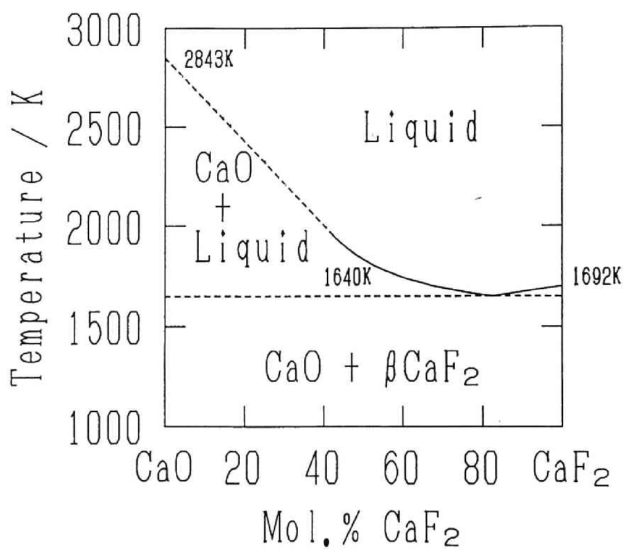
Figure 2.7: Phase diagram of the \text{CaF}_2 - \text{CaO} system [16].
