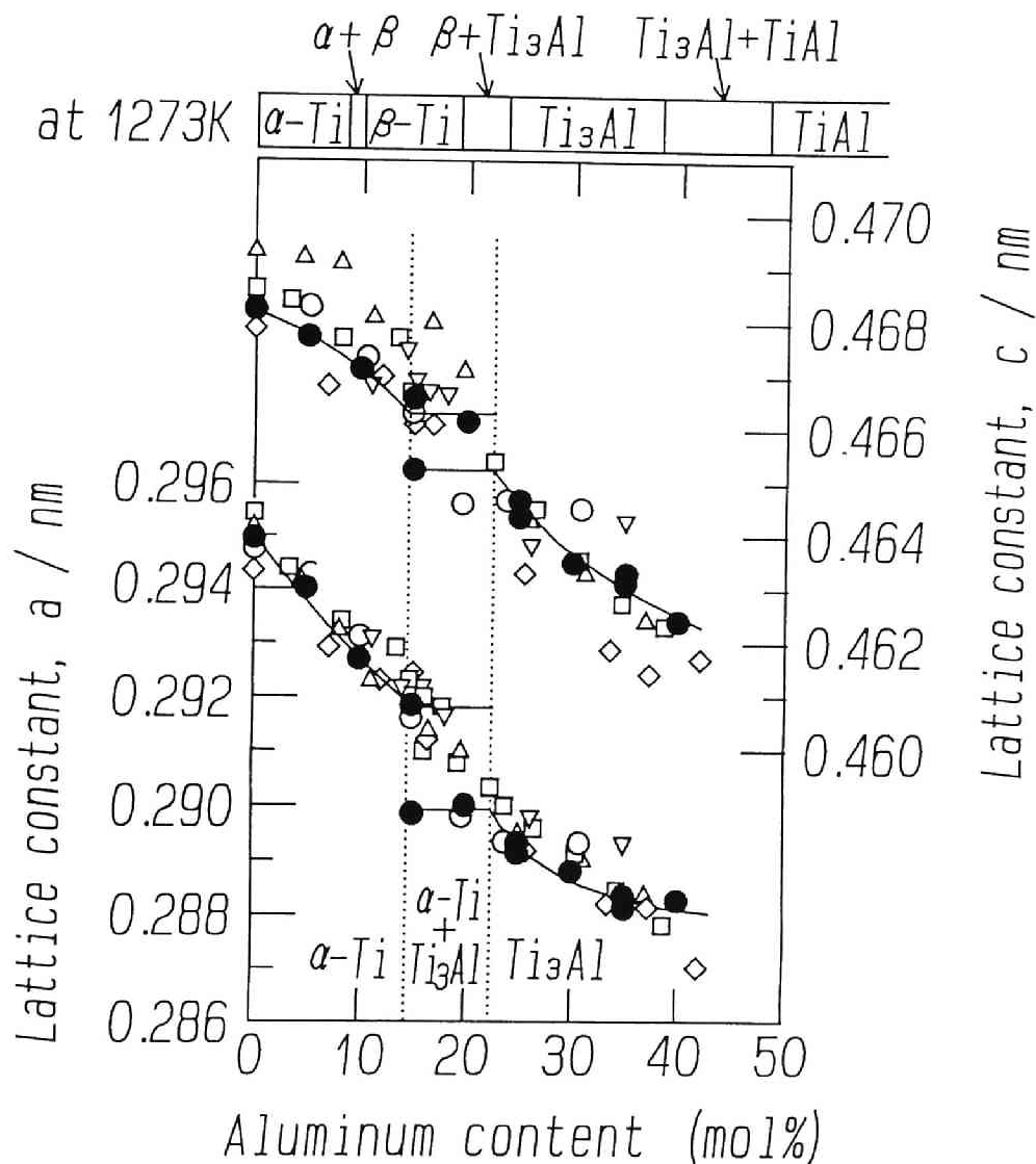
Figure 3.6: Lattice constants of the hexagonal phases after reduction by \text{CaH}_2 at 1273K for 43.2ks. The symbols in the figure are as follows; \bullet : This study by \text{CaH}_2 , \circ : Suzuki et al. by calcium vapor[7], \Delta : Ogden et al. [13], \diamond : Bumps et al. [14], \square : Clark et al. [15] and \nabla : Crossley[16].
