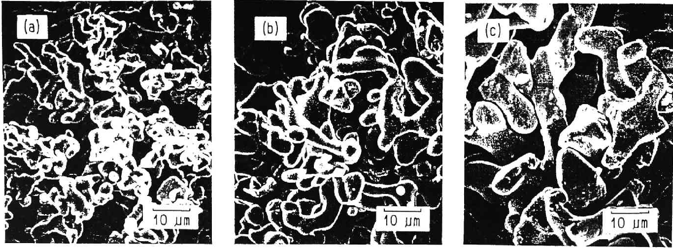
Figure 5.3: Scanning electron micrographs of titanium powders reduced by \text{CaH}_2 at 1273K for (a): 3.6ks, (b): 21.6ks and (c) 57.6ks. Calcium and \text{CaO} was removed by leaching before observation. The oxygen concentration of these powders were analyzed to be (a): 3400 ppm, (b): 2100 ppm and (c): 1500 ppm.
