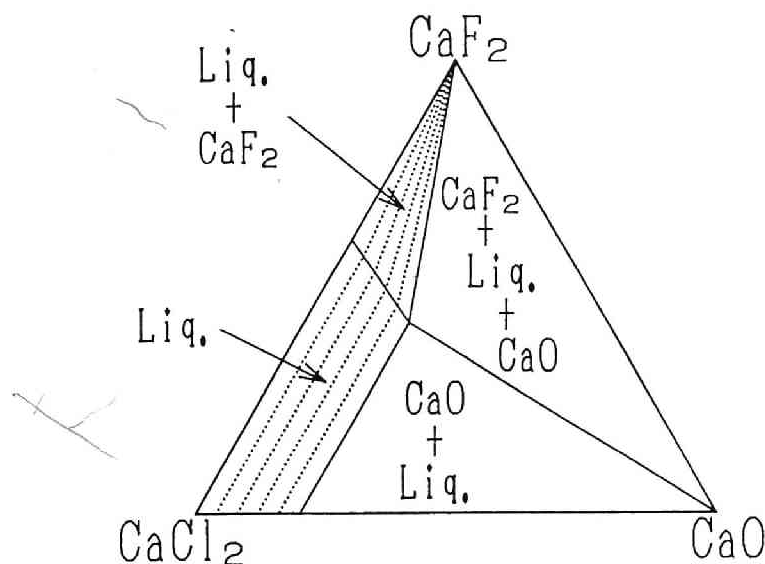
Figure 2.8: Qualitative phase diagram of the \text{CaCl}_2 - \text{CaF}_2 - \text{CaO} system at 1273K. Isoactivity lines for \text{CaO} are drawn as dotted lines
