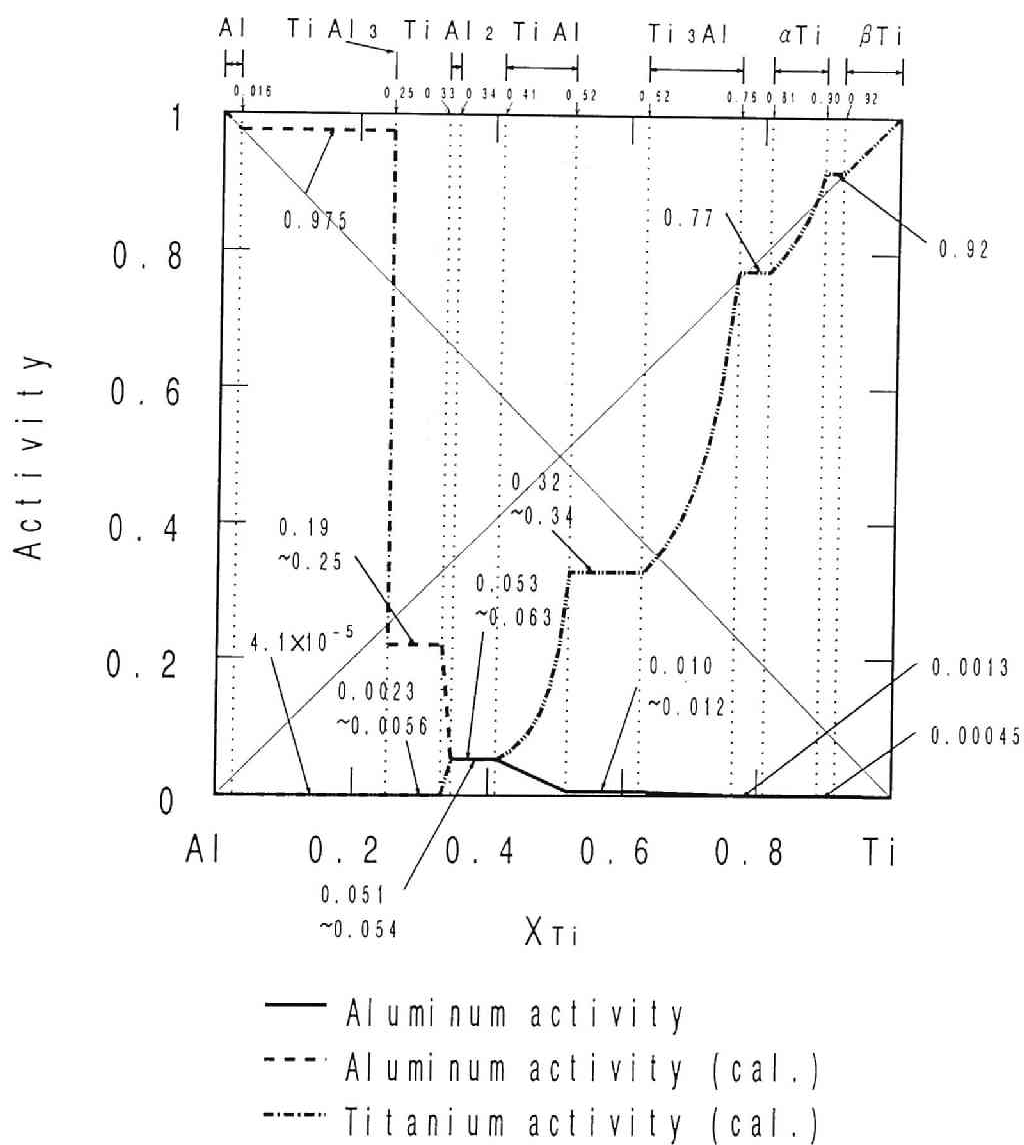
Figure 1.9: Composition dependence of activities in Ti-Al alloys at 1273K in linear scale.
