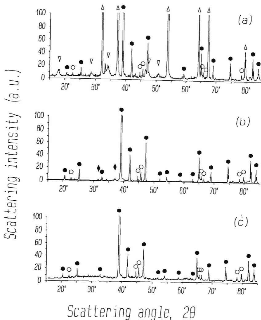
Figure 4.2: XRD patterns using \text{CuK}\alpha for the sample reduced at 1273K for 10.8ks from the oxide mixture with a ratio of \text{Al/Ti} = 3/1 . Pattern (a) was for the as-reduced specimen. (b) was for the same specimen after leaching in \text{CH}_3\text{COOH} aqueous solution. (c) was for the same specimen after the subsequent leaching in \text{HCl} aq. The symbols in the figure indicate \text{CaO} (Δ), \text{Ca(OH)}_2 (▽), \text{CaAl}_2 (◆), \text{TiAl}_2 (○) and \text{TiAl}_3 (●).
