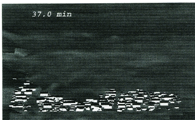
Photo 13 37 minutes after the earthquake ,the 3rd tsunami which exceeds 6m high covers the urban area.
