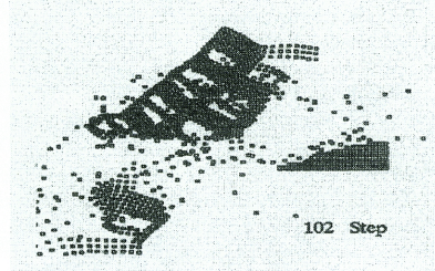
Photo 6 The result that the collapse of the brick structure analyzed by using D.E.M.
