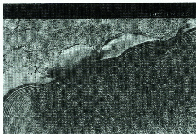
Photo 11 14 minutes after the earthquake, the first tsunami which exceeds 7m hits the southern end of the Kishu Peninsula.
