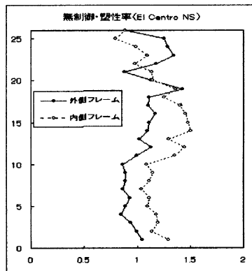
Fig. 2 Maximum Plastic Response Ratio (without active structural control system)
