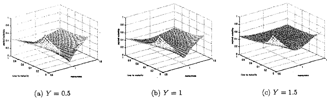
Figure 10: [G-CGMY Process & MEMM] Model ( b = 0, C = 0.05, G = 0.5, M = 0.5 )
