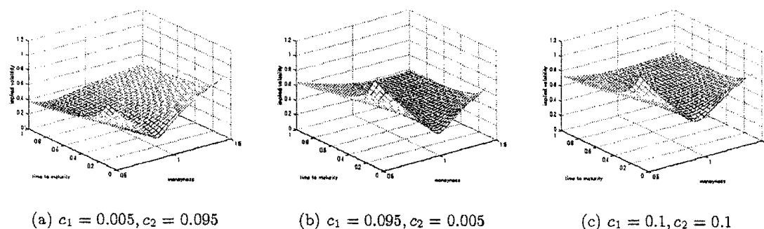
Figure 6: [G-Stable Process & MEMM] Model ( b = 0, \alpha = 1.2 )
