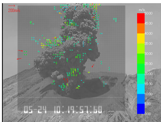
Fig. 3 A typical result of direct PIV analysis using the original images shown in Fig. 2. There are some erroneous vectors.
