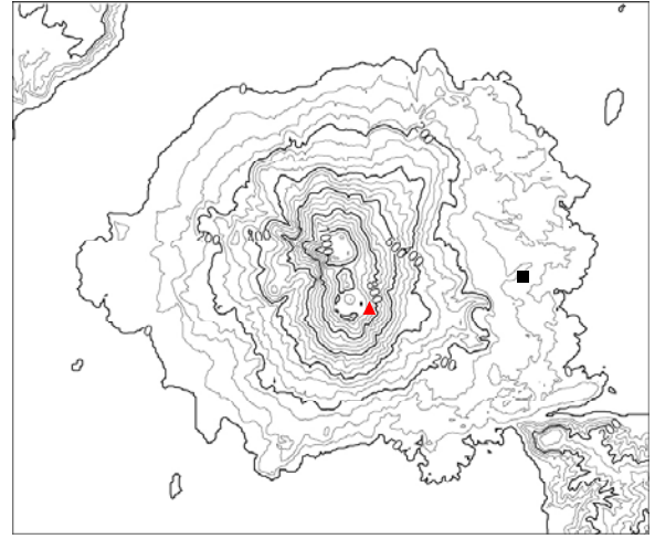
Fig. 1 Location of Showa crater (red triangle) and Kurokami observation site (black square).
