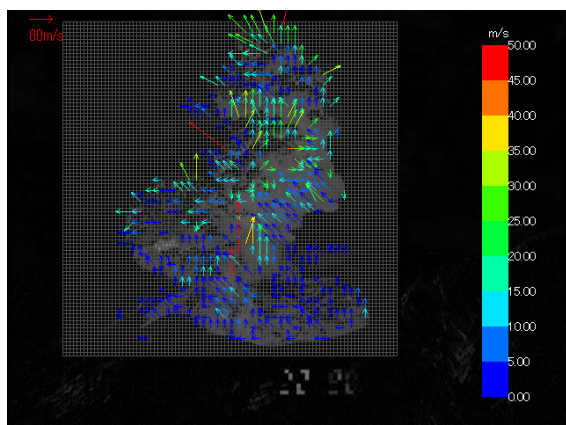
Fig. 4 A typical result of PIV analysis using the images that represent the difference from the initial image.
