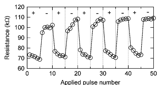
Fig. 6. Resistance switching behavior of the Ag-PCMO-Ti device. The PCMO film was deposited at the \text{Ca}(\text{DPM})_2/\text{THF} flow rate of 0.5 sccm and then annealed at 600 °C.
