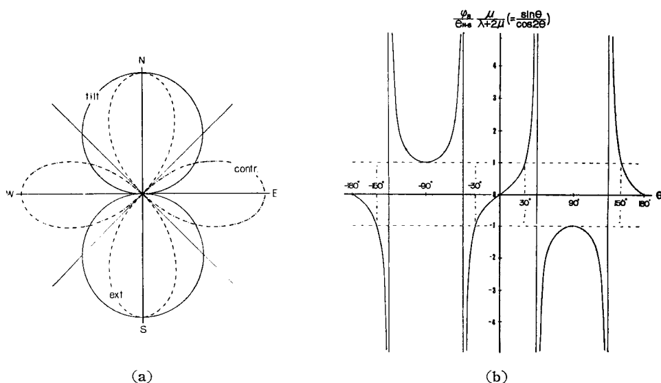
Fig. 2 (a) Diagram of linear strain and tilt in N-S component due to the direction of centre of point load, in the case of unit load and unit distance.
