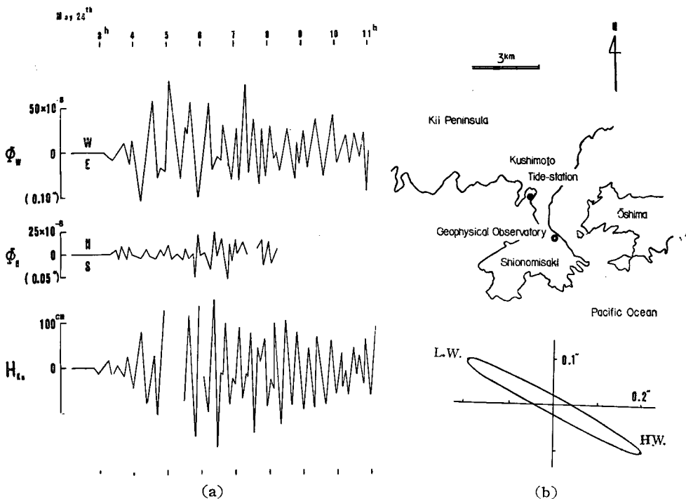
Fig. 8 (a) Oscillatory variations of ground tilt and water height due to the load of the Chile Tsunami observed at Shionomisaki observatory and Kushimoto tide-station.
