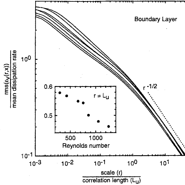
図 2: Root-mean-square fluctuation \sigma_{\varepsilon_v}(r) for boundary-layer turbulence as a function of the scale r . The ordinate is normalized by \langle \varepsilon_v(x) \rangle . The abscissa is normalized by L_u . The inset shows the dependence on the microscale Reynolds number Re_\lambda at r = L_u .
