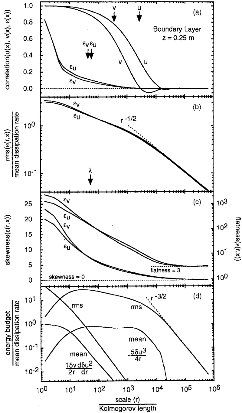
Fig. 1: Statistics as a function of the scale r normalized by the Kolmogorov length \eta . (a) Correlation functions \phi_{\epsilon_u}(r)/\phi_{\epsilon_u}(0) , \phi_{\epsilon_v}(r)/\phi_{\epsilon_v}(0) , \phi_u(r)/\phi_u(0) , and \phi_v(r)/\phi_v(0) . The arrows indicate the correlation lengths L_{\epsilon_u} , L_{\epsilon_v} , L_u , and L_v . (b) Root-mean-square fluctuations \sigma_{\epsilon_u}(r) and \sigma_{\epsilon_v}(r) . They are respectively normalized by \langle \epsilon_u(x) \rangle and \langle \epsilon_v(x) \rangle . The arrow indicates the Taylor microscale \lambda . (c) Skewness and flatness factors for \epsilon_u(r, x) and \epsilon_v(r, x) . (d) Averages and root-mean-square fluctuations of -5\delta u^3/4r and 15\nu\partial_r(\delta u^2)/2r coarse-grained over the scale r . They are respectively normalized by \langle \epsilon_v(x) \rangle and \langle \epsilon_u(x) \rangle .
