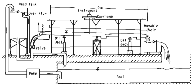
Fig. 9. Experimental flume.
