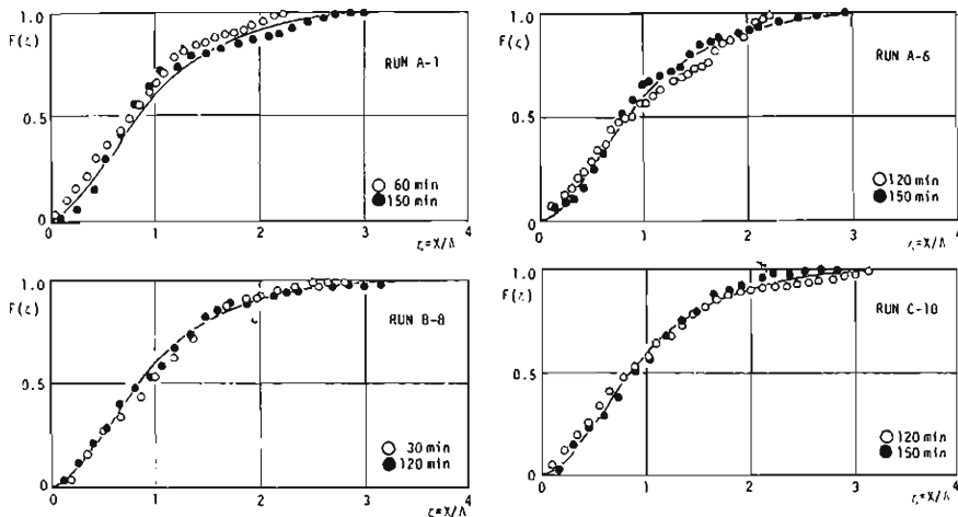
Fig. 18. Distribution of step length in duned beds.
