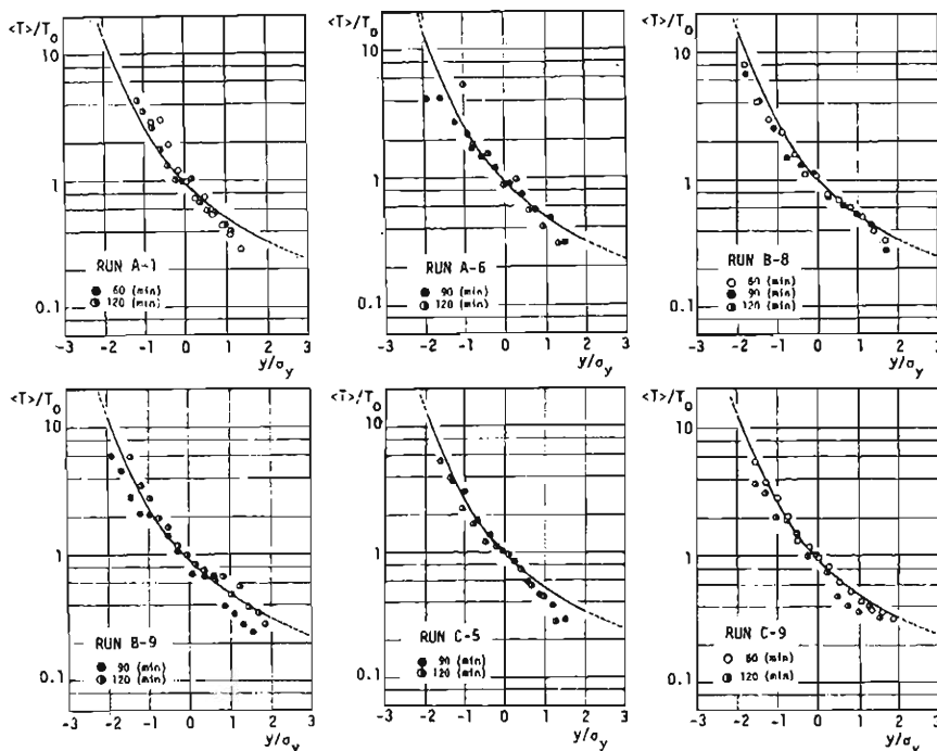
Fig. 11. Variation of conditional mean rest period in y -direction.
