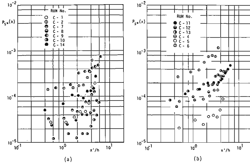
Fig. 3. Spatial variation of sediment pick-up rate over a simulated dune.
