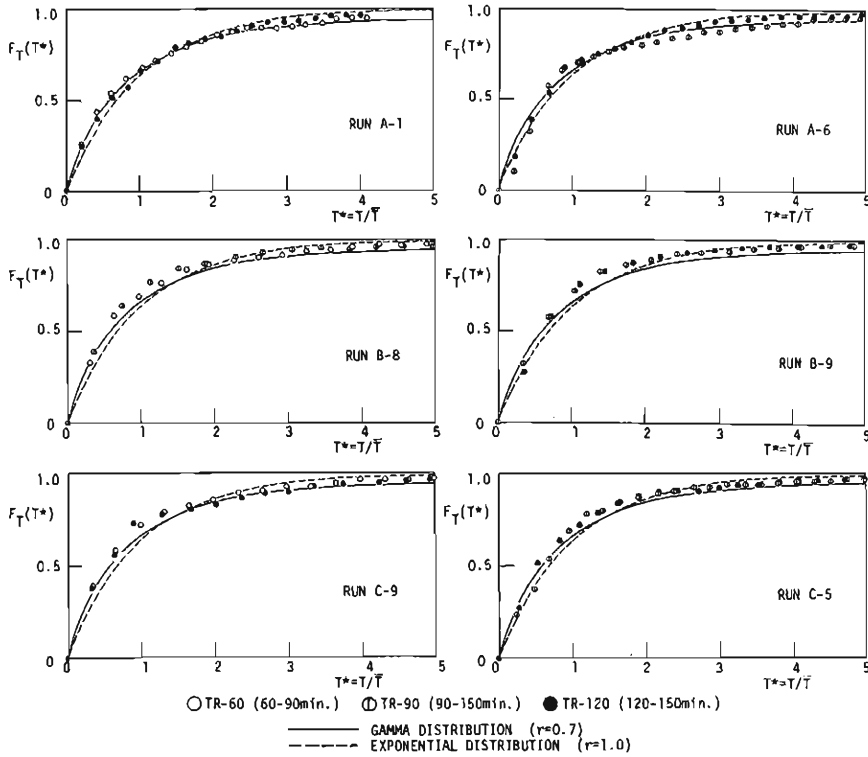
Fig. 15. Distribution of rest period in duned beds.
