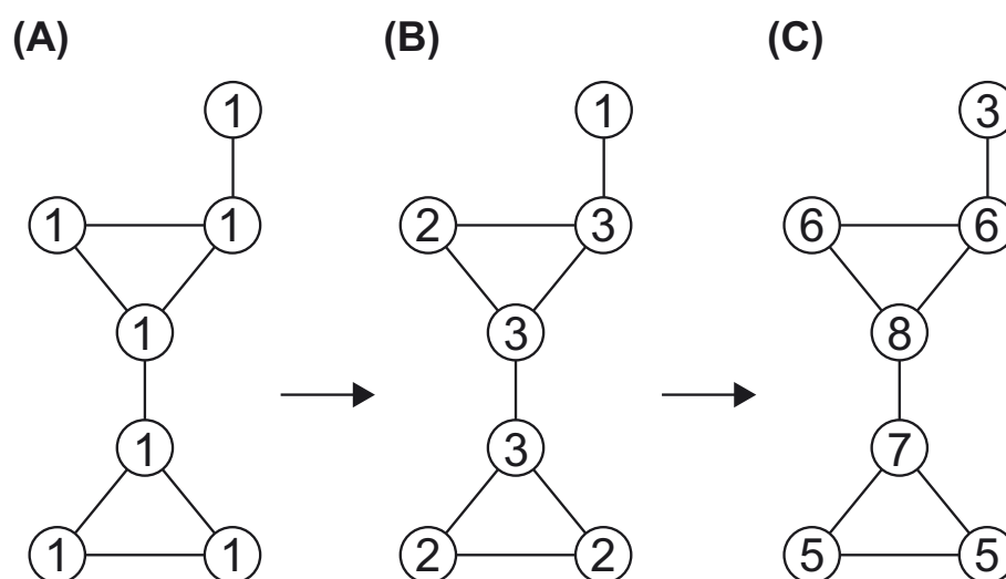
Figure 3 Example of calculation of Morgan index. (A) 1 is assigned to each vertex. (B) first iteration. (C) second iteration.
