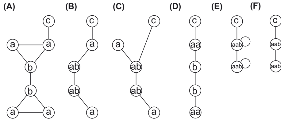
Figure 1 Example of contraction of identical edges. (A) Graph with 7 vertices and 8 edges. (B, C) Graphs contracted from graph (A) by GRAPHITOUR. (D) Graph contracted from graph (A) by our proposed method. (E) Graph contracted from graph (A) by substituting two edges ('a', 'a') and ('a', 'b') with 'aab'. (F) Graph contracted from graph (A) by substituting three vertices and the edges between the vertices with 'aab'.
