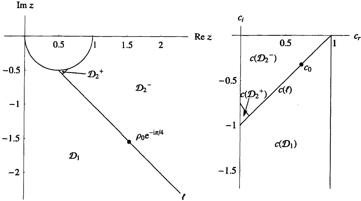
Figure 1: The sets D_1 , D_2^\pm and \ell of z , and the corresponding sets of c = 1 - 1/z .
