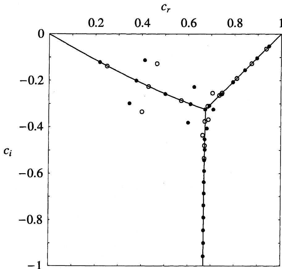
Figure 2: The Y-shaped contour obtained from (10)–(12), with c computed by Schmid & Henningson [15], [16] for R = 3000 ( \bullet ) and R = 2000 ( \circ ) when \alpha = 1 .
