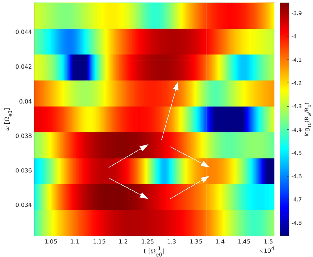
Figure 13. Dynamic spectrum for forward-propagating waves within t = 10159 \sim 15123 \Omega_{e0}^{-1} and \omega = 0.032 \sim 0.046 \Omega_{e0} at h = 100 c \Omega_{e0}^{-1} in a uniform background magnetic environment, where obvious merging and splitting of wave packets can be found, as indicated by white arrows.
