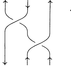
FIGURE 3. An example of b_3^\epsilon with s(b_3^\epsilon) = \epsilon = \downarrow\uparrow\uparrow and t(b_3^\epsilon) = \uparrow\downarrow\uparrow
