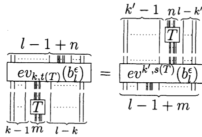
FIGURE 7. (T4): braid-tangle relation
