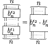
FIGURE 5. (T2): braids composition
