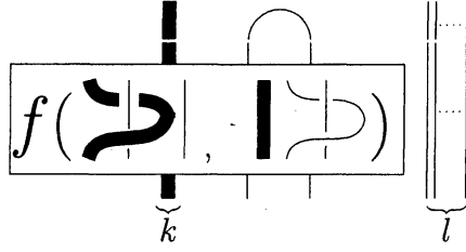
FIGURE 10. \sigma(a_{k,l}^\epsilon)
