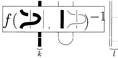
FIGURE 11. \sigma(c_{k,l}^\epsilon)
