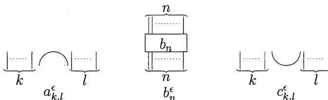
FIGURE 1. Topological picture of fundamental profinite tangles
