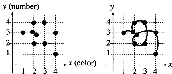
Figure 4: (a) Geometric view of a UNO-1 graph, where all the edges are omitted and (b) a Hamiltonian path in the UNO-1 graph.
