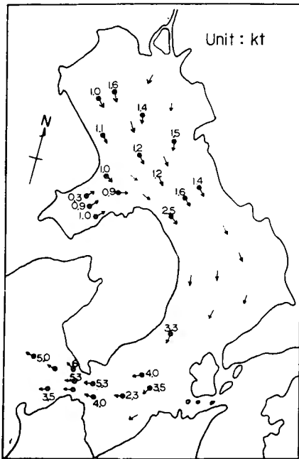
Fig. 2. Maximum tidal current in the ebb (Prototype).
