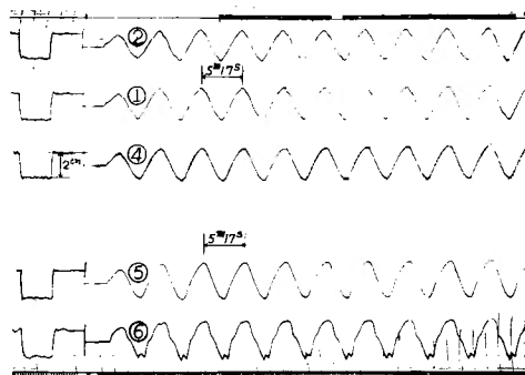
Fig. 8. Record of water level in the model.
