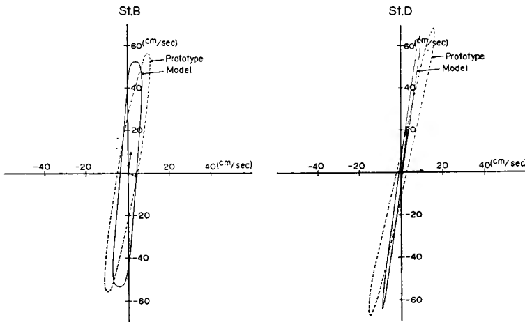
Fig. 10. Current ellipse.
