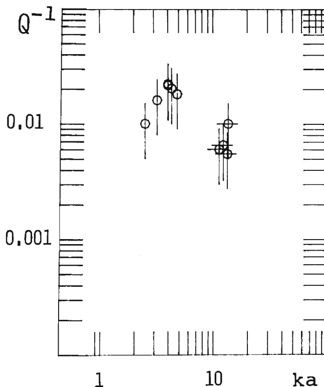
Fig. 8. Measured values of scattering attenuation ( Q^{-1} ). Bars denote the standard deviation.
