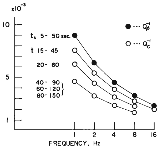
Fig. 1. Q_\epsilon^{-1} in various lapse time intervals and Q_\beta^{-1} for the Kinki district; t , lapse time; t_s , S-wave travel time. Note that Q_\epsilon^{-1} converges to Q_\beta^{-1} with the approach of the lapse time interval to the S travel time. (Reproduced from data listed in Tables 3 and 5 in Akamatsu's paper 6) .)
