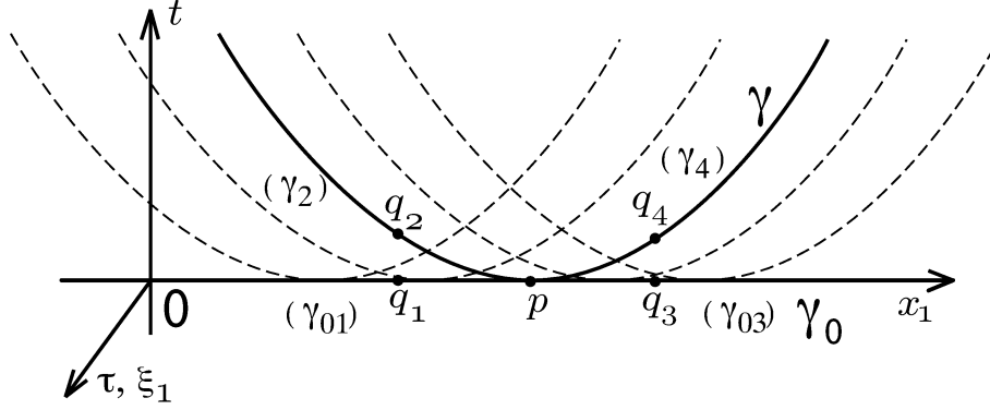
Figure 1. diffractive rays
