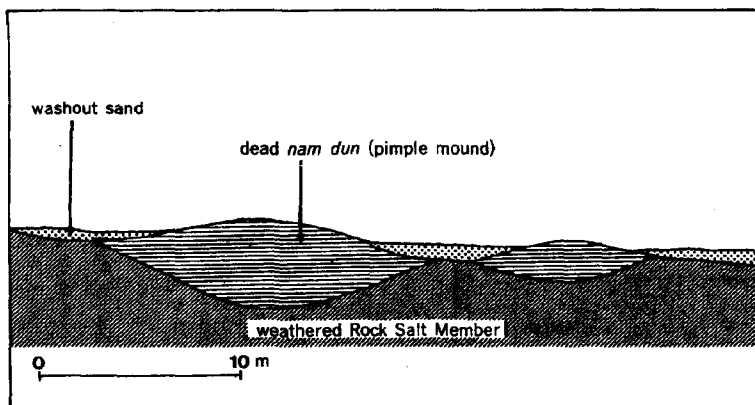
Fig. 12 A Schematic Cross Section of the Pimple Mound (Modified after Takaya et al. [1985])
