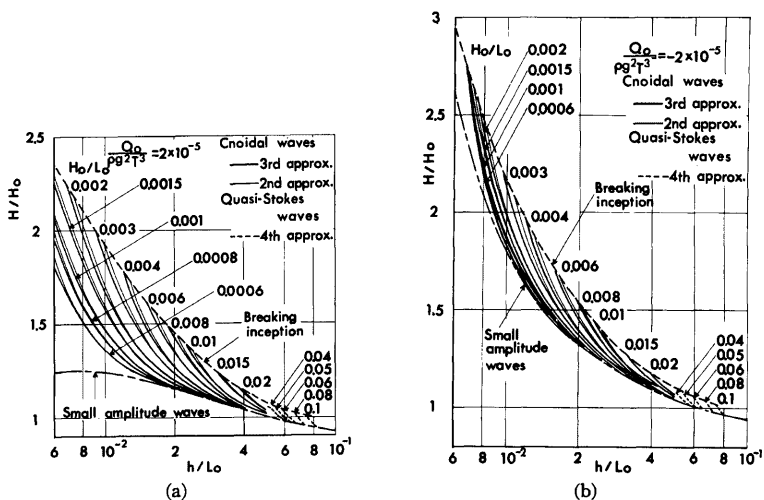
Fig. 4. Change of wave height with water depth under constant discharge.
