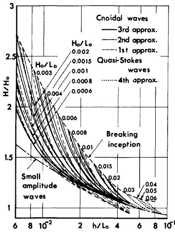
Fig. 1. Change of wave height with water depth on sloping beach.
