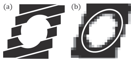
Fig. 1. Schematic illustration of coarse gaining for the approximation of discontinuous brittle deformation using a homogeneous one. 粗視化で不連続変形を一様変形で近似する例.
