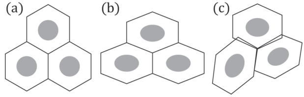
Fig. 10. Schematic illustration of the homogeneous and heterogeneous deformations of a crystalline aggregate. (a) The configuration of three crystal grains before deformation. (b) After homogeneous deformation. (c) After heterogeneous one. 多結晶体 (a) が一樣変形する場合と (b), そうでない場合 (c) を示す模式図。
