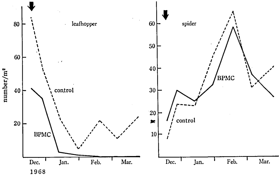
Fig. 1. Effect of 4% BPMC-granular formulation (3kg/1000m 2 ) on numbers of green rice leafhopper (left) and spider (right) in the paddy field. The left-up arrow denotes the time of insecticidal treatment.
