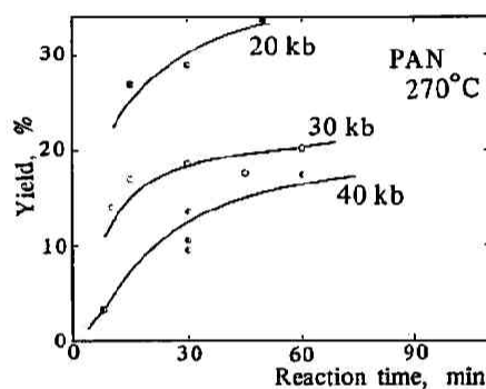
Fig. 15 Dependence of the yield on reaction time at 270°C
