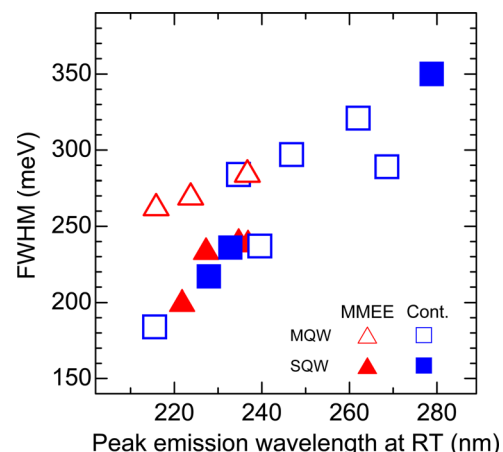
FIG. 4. (Color online) Variation in the PL line width of QWs at 8.5 K with emission wavelength at RT.
