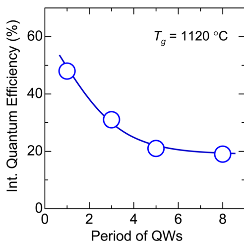
FIG. 5. (Color online) Variation of IQE due to QW period in 1.5 nm thick \text{Al}_{0.50}\text{Ga}_{0.50}\text{N}/\text{AlN} QWs grown by the continuous method.
