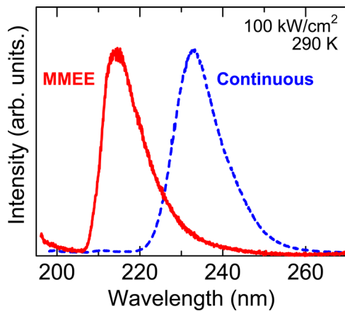
FIG. 2. (Color online) RT PL spectra of AlGaN/AlN SQWs fabricated by MMEE and continuous method under the same growth conditions except for the source-supply sequence.
