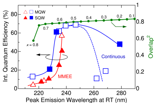
FIG. 3. (Color online) Summary of IQEs with emission wavelength for QWs grown by MMEE or continuous method. Calculated square overlap is also shown. Numbers in italics are Al compositions.
