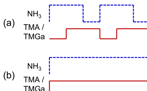
FIG. 1. (Color online) Sequence profile of \text{NH}_3 and metalorganic sources (TMA and TMGa) for (a) MMEE and (b) continuous methods.
