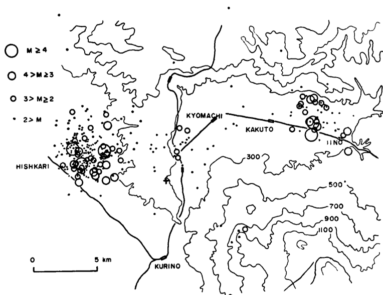
Fig. 3. Epicentral distribution of earthquakes occurred in and around Kakuto caldera, August 1978–December 1979.
