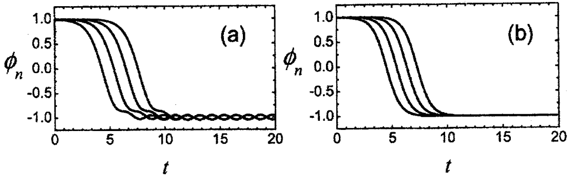
Fig. 2. Trajectories of particles (a) in the model of Eq. (32) with h = 0.7 when the kink moves with a steady velocity v^* (see Fig. 1(c), bottom panel) and (b) for the continuum \phi^4 kink.
