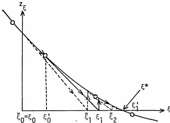
Figure 7.2. Illustration of computational processes of the Dinkelbach method and Algorithm B. (Solid arrows indicate Algorithm B and broken arrows indicate the Dinkelbach method.)
