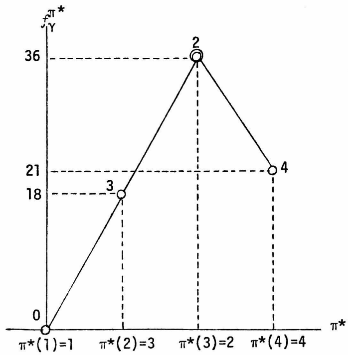
Figure 3.3. An optimal solution \pi^* .
