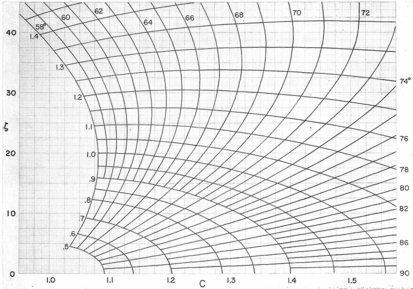
Chart 1. \zeta , 0^\circ to 45^\circ ; C , 0.95 to 1.575.
