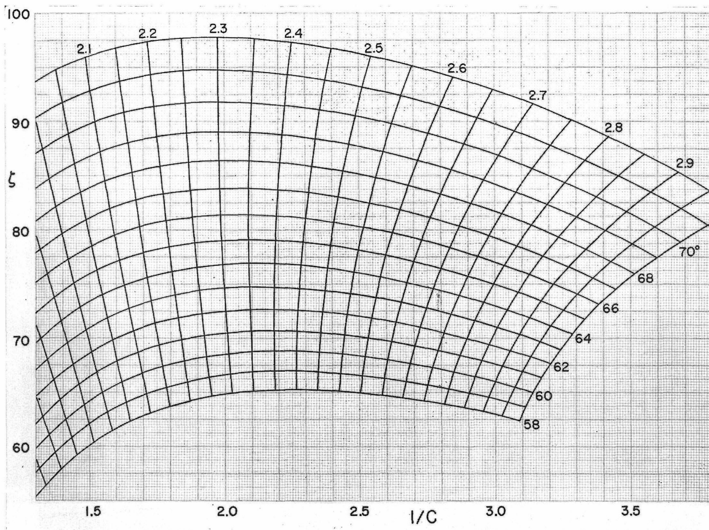
Chart 4. \zeta , 55° to 100°; 1/C , 1.3 to 3.8.
