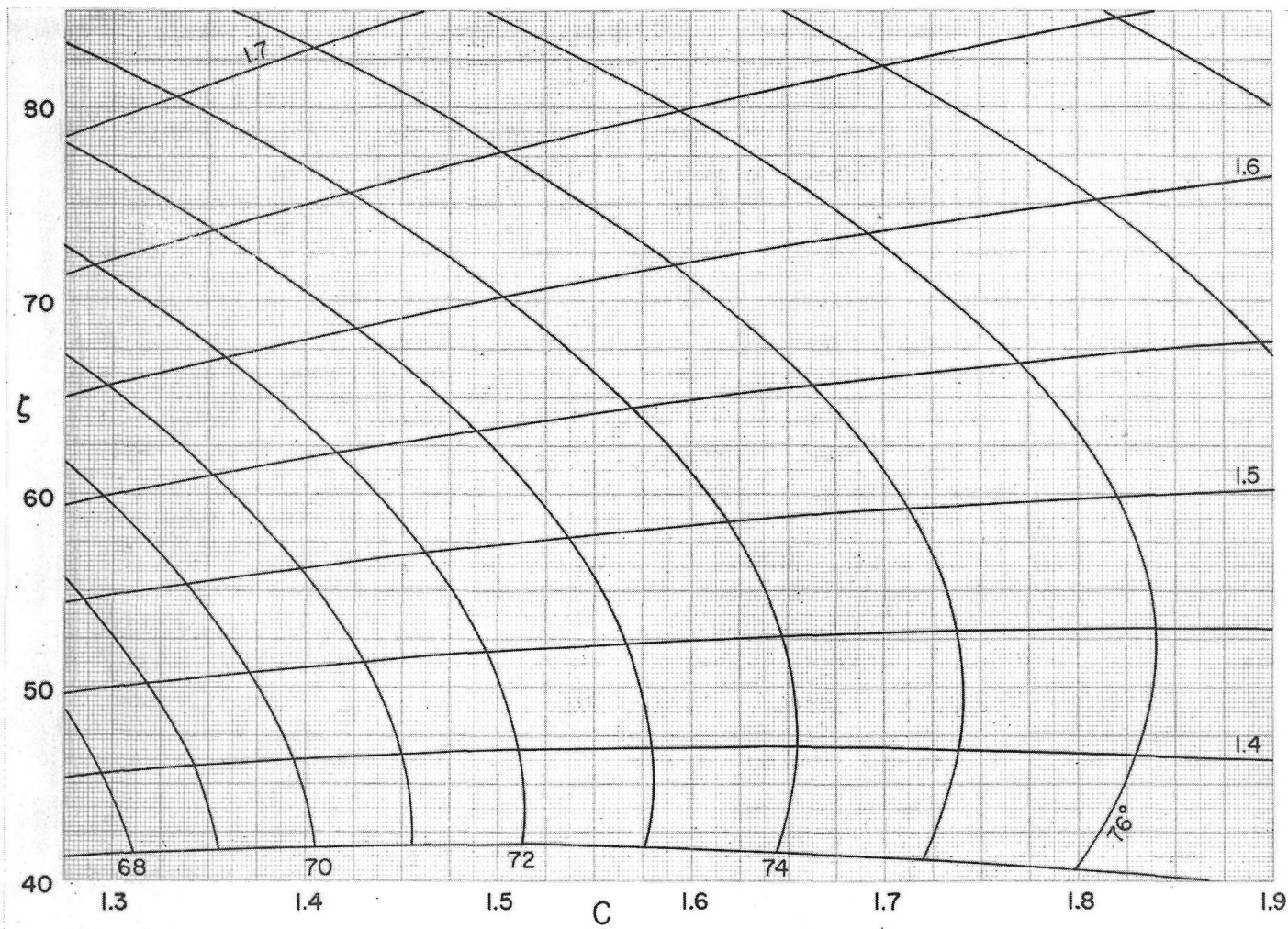
Chart 6. \zeta , 40^\circ to 85^\circ ; C , 1.275 to 1.9.
