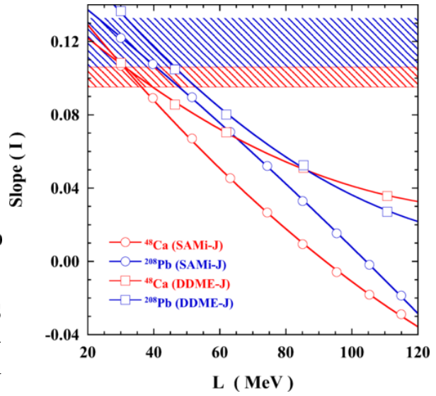
Figure 1.6: Correlation between the symmetry energy parameter L and the slope of the IS-IV density curve. The shaded areas show the experimental uncertainties. The black try energy parameter L and the slope of the solid curve gives the experimental trajectory. The dashed line corresponds to the experimental slopes obtained for ^{48}\text{Ca} and constant IV density limit \rho_{\text{IV}} = \rho_{\text{IV}}(N - Z)/A . The colored solid curves are calculations with the SAMi-J families [23]. The slopes, shown by the colored dashed lines, are evaluated at the crossing points with the constant IV trajectory. Taken from Ref. [21].
