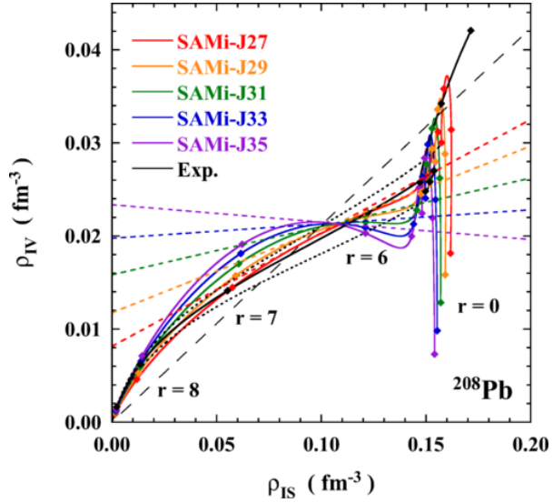
Figure 1.5: Trajectory in a 2D plot of IS and IV densities of ^{208}\text{Pb} . The experimental trajectory is given by the black solid curve sandwiched between two dotted lines. The area between the two dotted lines shows the experimental uncertainties. The black try energy parameter L and the slope of the solid curve gives the experimental trajectory. The dashed line corresponds to the experimental slopes obtained for ^{48}\text{Ca} and constant IV density limit \rho_{\text{IV}} = \rho_{\text{IV}}(N - Z)/A . The colored solid curves are calculations with the SAMi-J families [23]. The slopes, shown by the colored dashed lines, are evaluated at the crossing points with the constant IV trajectory. Taken from Ref. [21].
