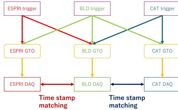
Figure 2.11: DAQ diagram.
