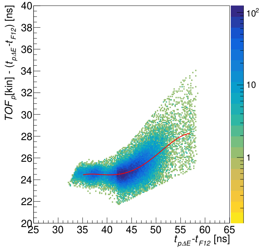
Figure 3.15: 2D spectrum of (t_{p\Delta E} - t_{12}) versus t_{\text{off}} = TOF_p[\text{kin}] - (t_{p\Delta E} - t_{12}) . In the region of (t_{p\Delta E} - t_{12}) < 42 \text{ ns} , the elastic events were selected using the NaI(Tl) calorimeters. The red line shows the fitting function in the form of a fourth-order polynomial function.
