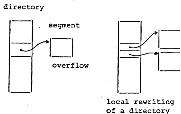
(b) An adaptive segmentation scheme
