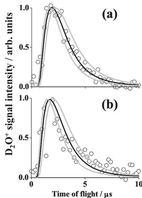
FIG. 5. (a) TOF spectrum of \text{D}_2\text{O}(v=0) formed by 157 nm photoirradiation of ASW( \text{D}_2\text{O} ) at 90 K, monitored by 2+1 REMPI via the line at 248.057 nm of the \text{C}-\text{X} 0_0^0 band. The solid curve is a fit to the data derived assuming T_{\text{trans}}=1800 K. (b) TOF spectrum of \text{D}_2\text{O}(v=0) formed by 193 nm photoirradiation of the \text{D}_2\text{O}:\text{H}_2\text{S} mixed ice sample at 90 K, monitored by (2+1) REMPI via the line at 247.865 nm, which is mainly the 1_{01}-2_{20} transition of the \text{C}-\text{X} 0_0^0 band. The solid curve is a fit to the data derived assuming T_{\text{trans}}=2250 K. The two gray curves show the range spanned by the error bars quoted in Table I.
