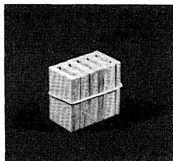
Fig. 2. Binding of wood blocks for decay test.
