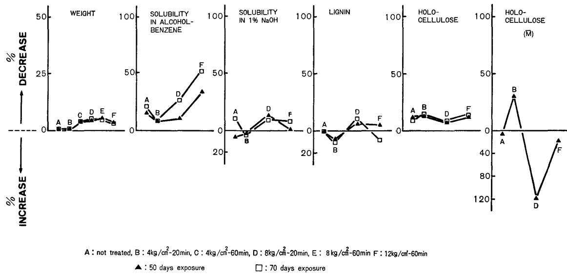
Fig. 12. Chemical changes in PC-treated wood blocks of Pinus densiflora after exposure to decay fungus Coriolus versicolor in comparison with non-inoculated wood.
