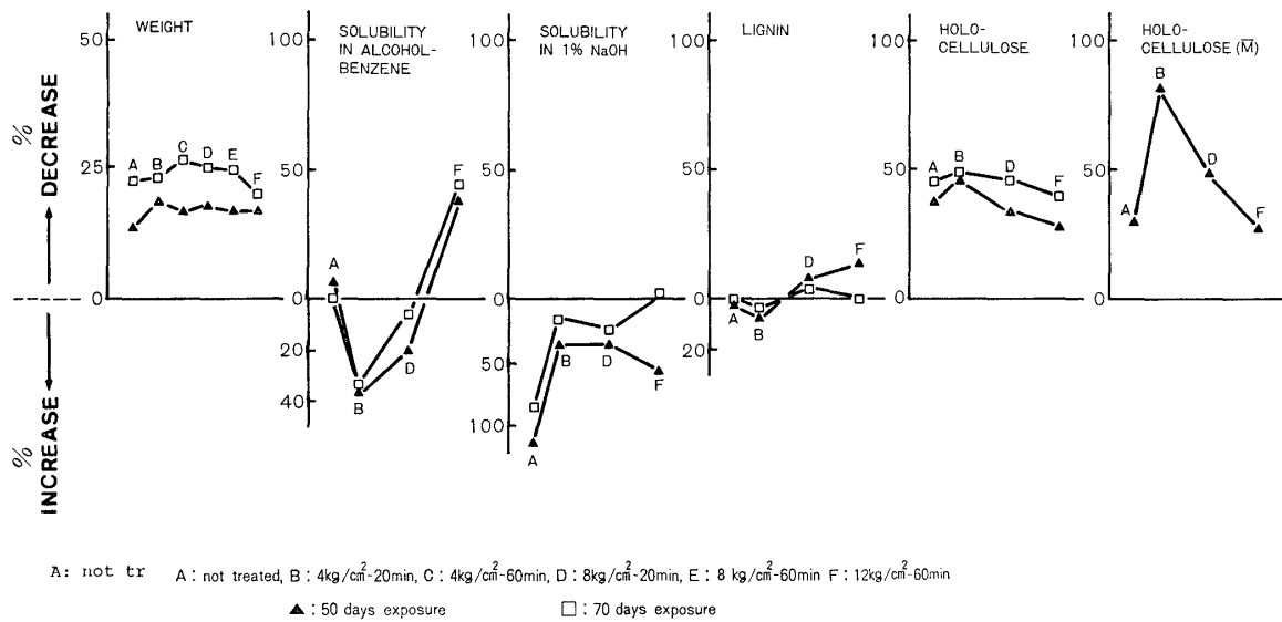
Fig. 14. Chemical changes in PC-treated wood bloccks of Pinus densiflora after exposure to decay fungus Tyromyces palustris in comparison with non-inoculated wood.
